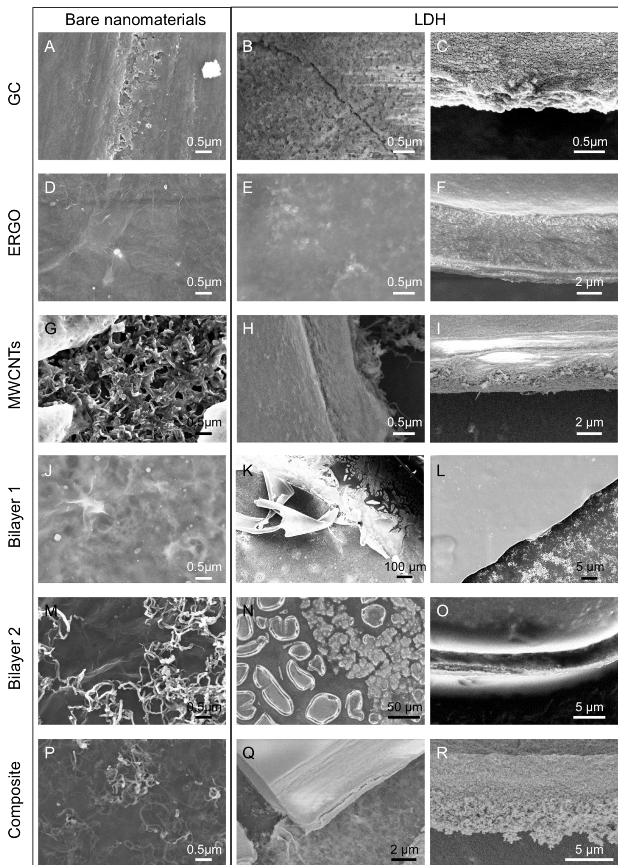
Figure 4. SEM images for bare GC (A), ERGO/GC (D), MWCNTs/GC (G), Bilayer1/GC (J), Bilayer2/GC (M), Composite/GC (P), LDH/GC (B) and (C), LDH/ERGO/GC (E) and (F), LDH/MWCNTs/GC (H) and (I), LDH/Bilayer1/GC (K) and (L), LDH/Bilayer2/GC (N) and (O) and LDH/Composite/GC (Q) and (R).
