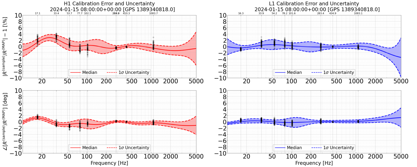
Figure 2. LIGO Hanford (left) and Livingston (right) frequency-dependent calibration error for a 1 hr time period in O4a starting at 2024 January 15 08:00:00 UTC. The magnitude of the calibration error is shown in the top plots, and the phase of the calibration error (in units of degrees) is shown in the bottom plots. The median systematic error of the calibration is given by the solid line. The 1\sigma uncertainty on this systematic error is given by the dotted lines. The black dots overlaid on the figure at specific frequencies are direct measurements of the calibration error at a specific frequency during this 1 hr time period. These measurements are made using sinusoidal injections with the photon-calibrator system. These uncertainties are representative of typical LIGO calibration uncertainties throughout O4a.
