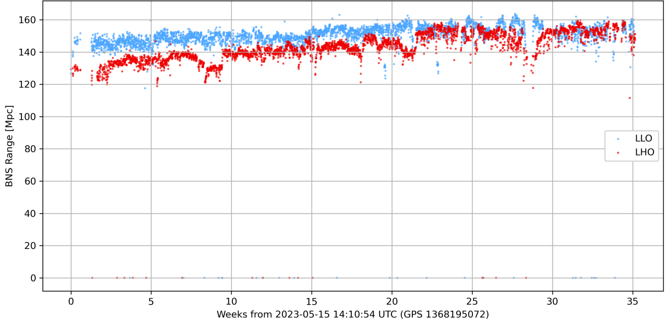
Figure 1. BNS inspiral range over time for O4a. Each point corresponds to a time interval of 4096 s, corresponding to the time range of one strain data file. The fast Fourier transform window length used is 8 s with a 4 s overlap. These inspiral range values are stored as metadata for each file in the GWOSC database and are accessible via the GWOSC website.
