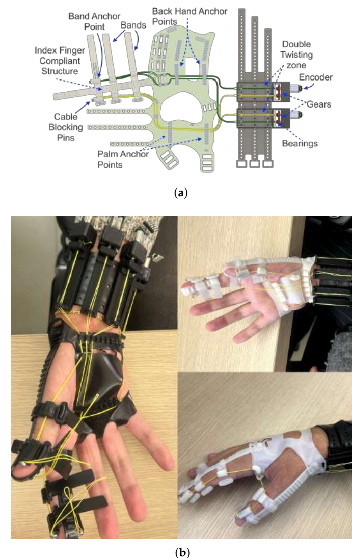
Figure 3. Soft glove prototype. (a) CAD model. (b) The glove worn by an end user.
