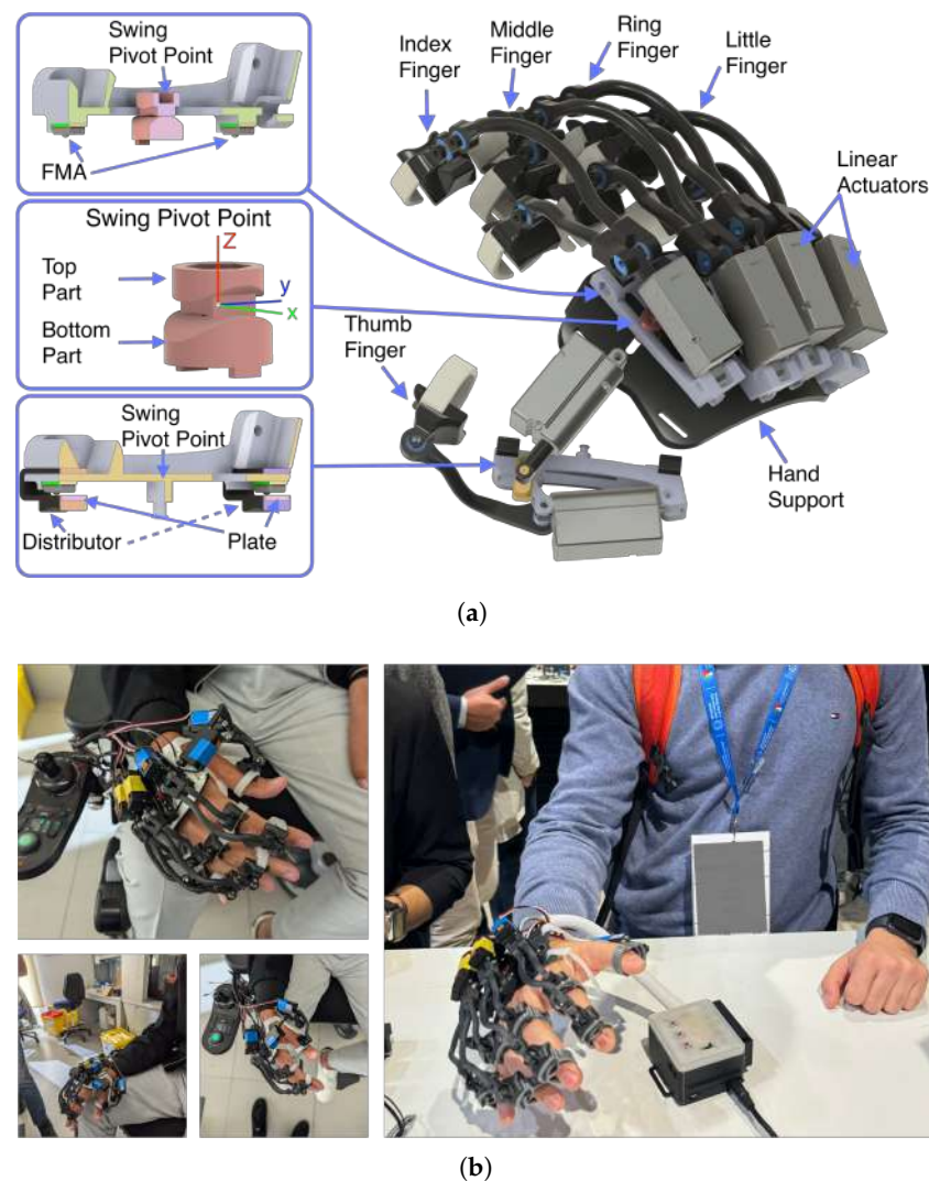
Figure 2. Rigid exoskeleton. (a) CAD model. (b) The hand exoskeleton worn by end users.
