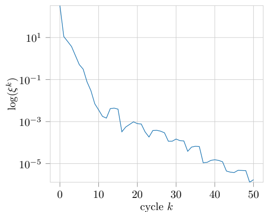
Figure 3: Logarithm of the measure of infeasibility \xi^k .
