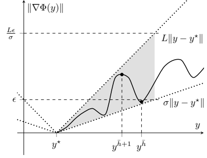
Figure 7: Representation of the results of Lemma 12.
