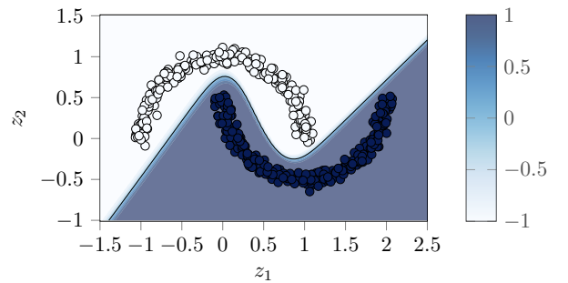
Figure 5: Two moons dataset. Blue dots represent points with label -1 and white dots points with label 1 . Colored regions represent the output of the classifier (20) resulting from the solution of (22) provided by ASYMM. The color of the regions is associated to a number as in the color bar.
