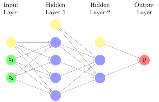
Figure 4: Graphical representation of the Neural Network used as classifier. In green the input units, in blue the hidden units, in red the output unit and in yellow the bias units.
