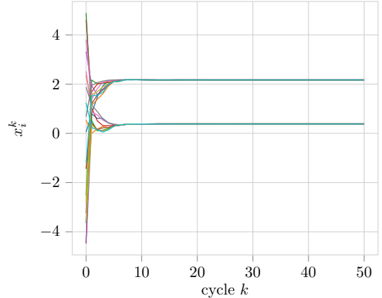
Figure 2: Evolution of the local decision variables x_i^k .
