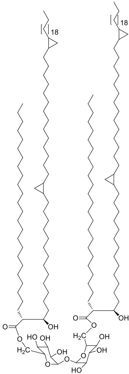
Trehalose-6,6'-di- \alpha -mycolate (TDM)
