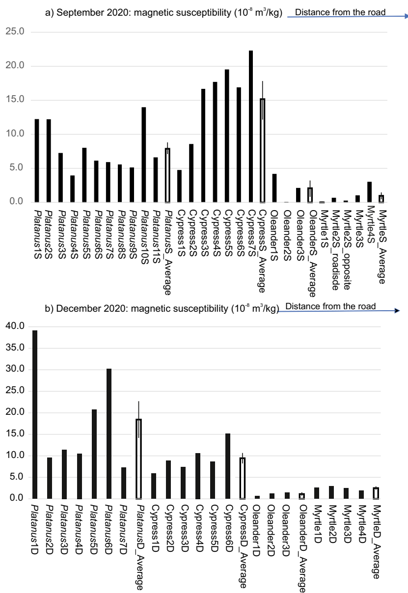
Fig. 2. Histograms of mass magnetic susceptibility of plant leaves, sampled in (a) September, suffix “S” and (b) December, suffix “D”: black bars = individual trees, white bars = site averages, with standard errors. The species are ordered from left to right, at increasing distances from the road. Myrtle 2 was sampled in September on both directions with respect to the road.
