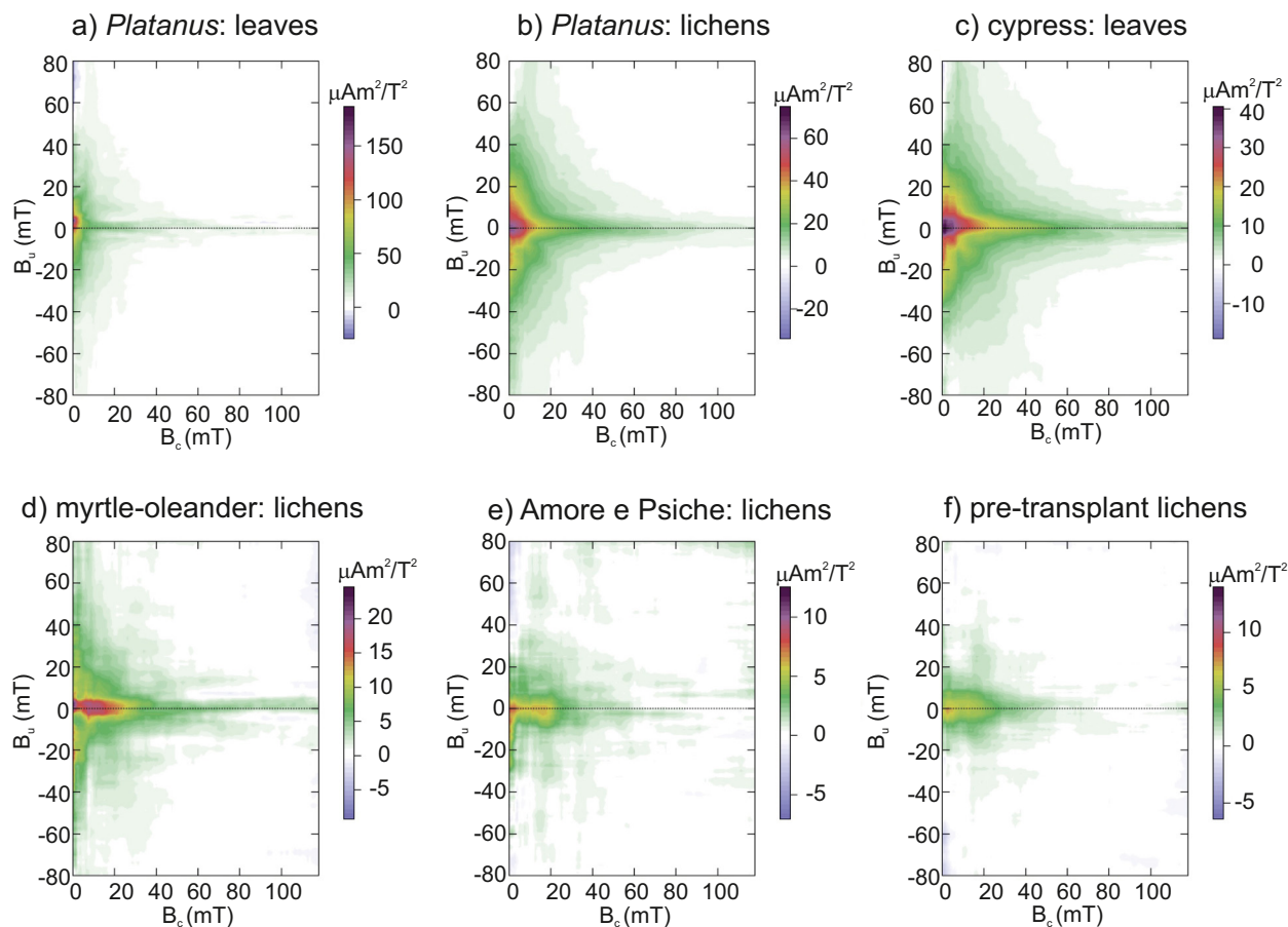
Fig. 4. FORC diagrams, for September leaves (a, c) and lichens (b, d, e, f): multidomain (MD) features prevail for the samples exposed outdoor and near the Lungotevere Farnesina busy road, while single domain (SD) characteristics emerge for the unexposed samples and for those exposed at higher distance from the road and inside the Amore e Psiche Hall. B_u is the interaction field, B_c the coercivity.
