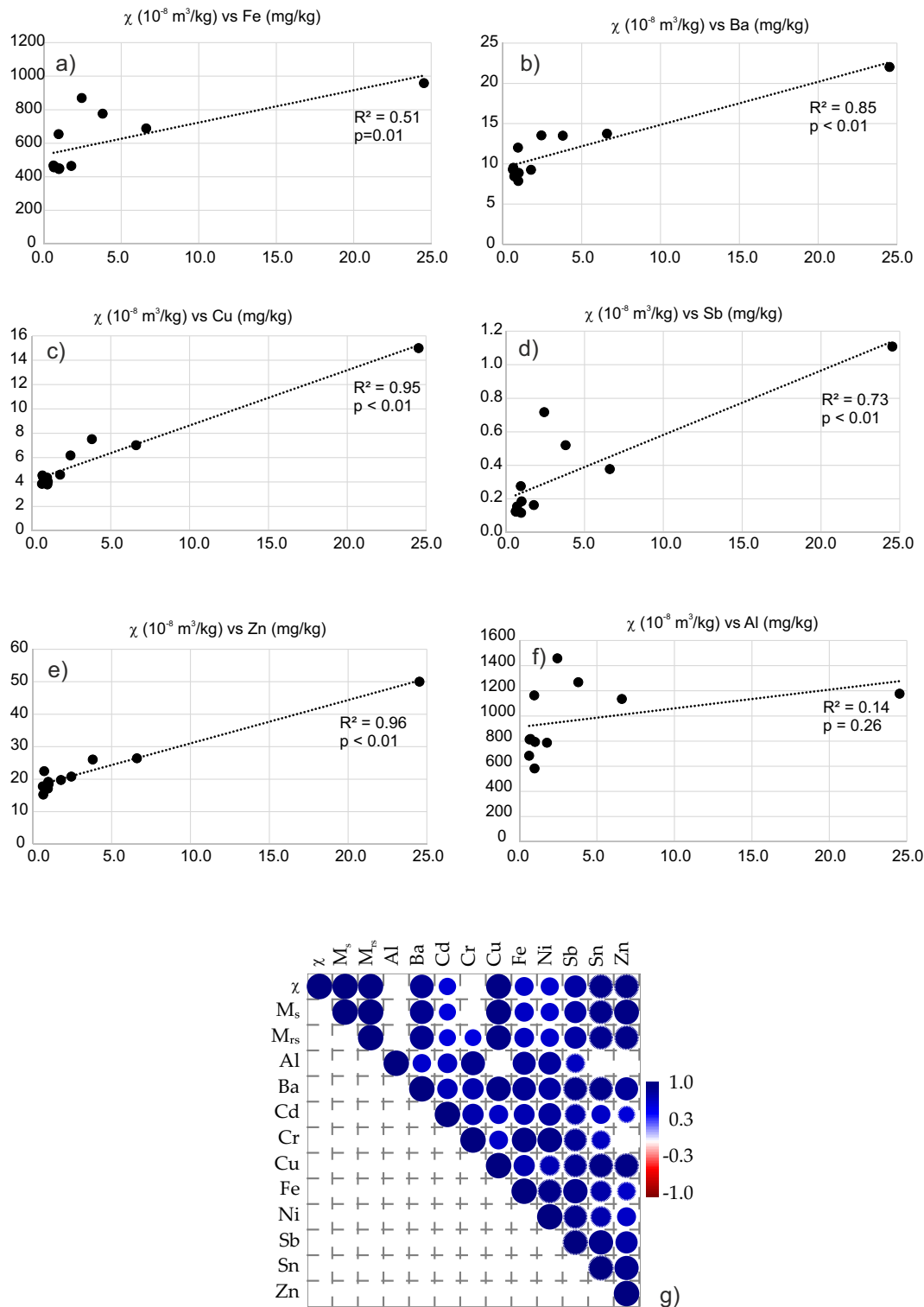
Fig. 6. Selected linear correlations between magnetic susceptibility ( \chi ) of lichens and element concentration (a, Fe; b, Ba, c, Cu; d, Sb; e, Zn; f, Al): all the elements but Al and Cr significantly correlated with \chi , at 95% confidence level. g) correlation plot of concentration dependent magnetic parameters and element concentration: the circle dimension represents the value of r, the linear correlation parameter, in blue when positive.
