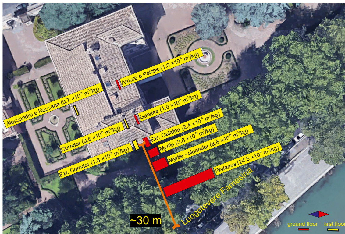
Fig. 7. Modified Google Earth aerial view of Villa Farnesina: the magnetic susceptibility values of lichen transplants are superimposed to the sampling sites as histograms. The magnetic susceptibility values decay with the distance from the road, that was evaluated by means of the proper Google Earth function and verified through the measurement with a laser telemeter.
