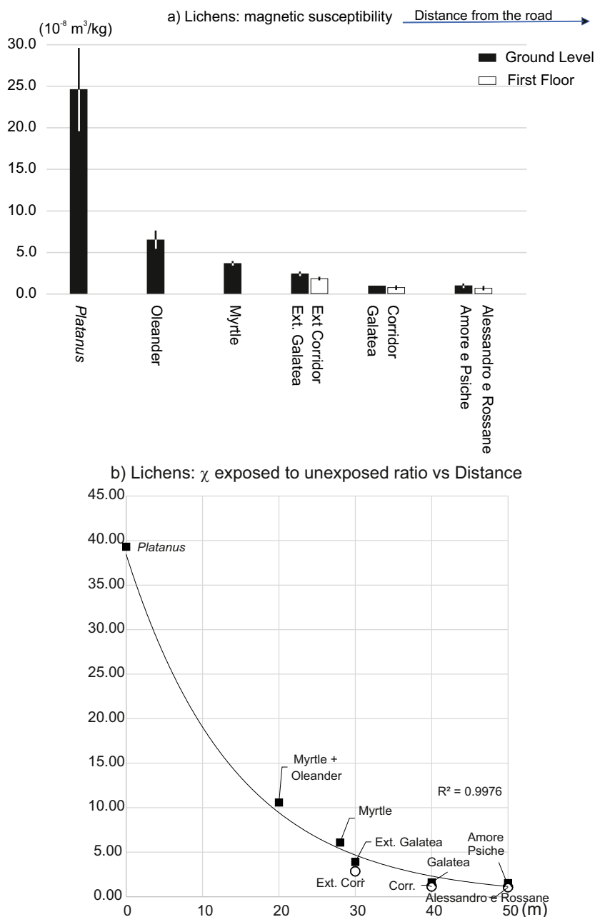
Fig. 5. The variability of lichens' magnetic susceptibility with the distance from the road: (a) average values and standard errors of mass magnetic susceptibility of lichens exposed for three months, black bars for samples on the ground floor, white for the first floor; (b) exponential decay of the magnetic susceptibility ( \chi ) ratio vs distance from the road, calculated as the magnetic susceptibility of exposed transplants normalized to the average value of the unexposed samples. Distances were evaluated by means of the proper Google Earth function, and successively verified through laser telemeter measurements.
