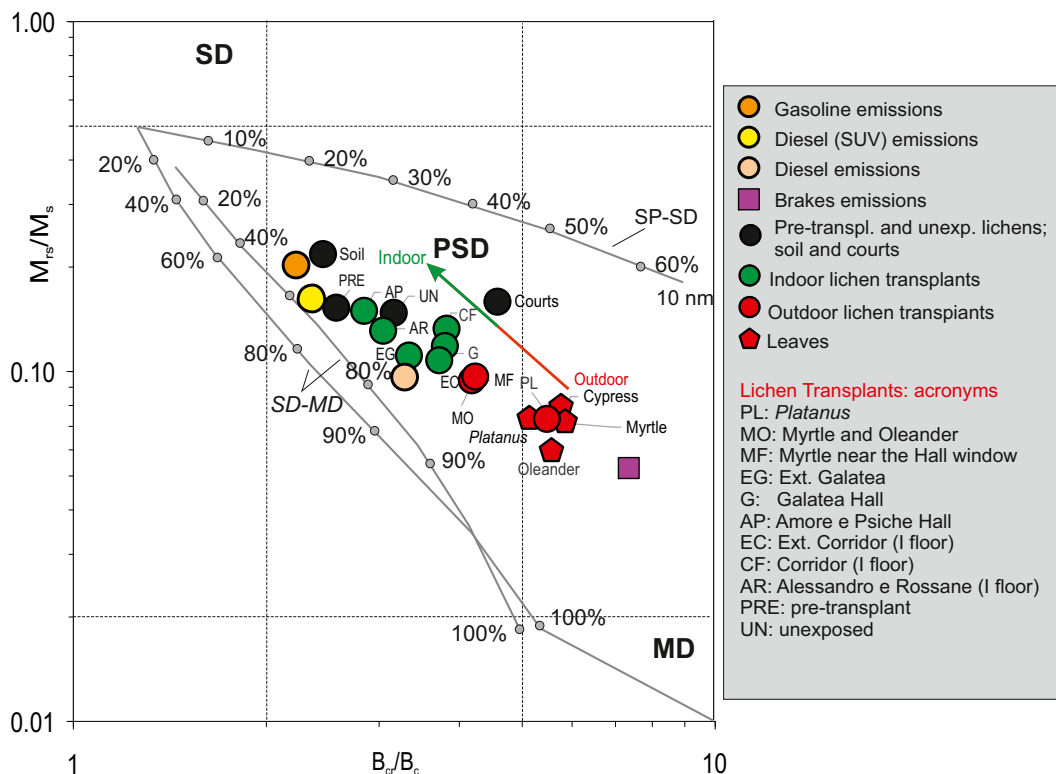
Fig. 3. Bilogarithmic “Day plot” (Day et al., 1977) of the site averaged hysteresis ratios for leaves and lichen transplants (pentagons and circles, respectively; red symbols outdoor samples, green circles indoor lichens), reported together with the average points for different kinds of fuel exhaust (orange, yellow and pink circles) and brake dust particles (purple square) calculated from Sagnotti et al., 2009. The SD (single domain), PSD (pseudo-single domain) and MD (multidomain) fields and the theoretical mixing trends for SD-MD and SP-SD pure magnetite particles (SP, superparamagnetic) are from Dunlop (2002a, 2002b). Unexposed, pre-transplant, soil of the gardens and court samples are reported as black circles. The outdoor samples are located at the middle-right side of the plot, near the brakes data, while the indoor transplants fall in the central part of the plot, close to the unexposed and pre-transplant control samples.
