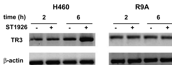
Figure 9. RT-PCR analysis of TR3 expression in H460 and R9A cell lines. RNA was isolated after 2 or 6 hours of treatment with solvent (–) or ST1926 (0.2 μM for H460 and 20 μM for R9A cells). Amplification products with primers for TR3 and β-actin, separated on agarose gel, are shown.
