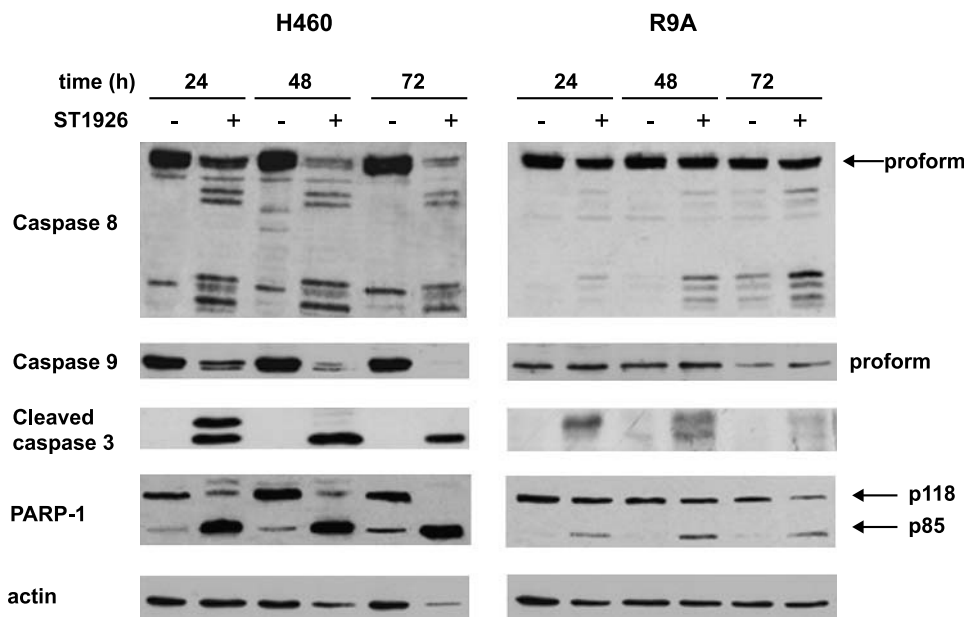
Figure 5. Cleavage of caspases and PARP-1 in cells exposed to ST1926. Western blot analysis with specific antibodies was performed after 24, 48, and 72 hours of exposure to 0.2 \mu M and 20 \mu M ST1926 in H460 and R9A cells, respectively ( IC_{80} at 72 hours). Actin is shown as a control for protein loading.
