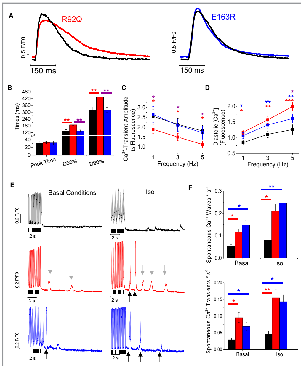
Figure 4. Intracellular \text{Ca}^{2+} measurements in intact ventricular cardiomyocytes. A, Representative superimposed \text{Ca}^{2+} transients elicited at 1 Hz in wild-type (WT) and R92Q cardiomyocytes (left) and WT and E163R cells (right). B, Time from stimulus to peak (Peak Time), time from peak to 50% and 90% decay of \text{Ca}^{2+} transients (D50% and D90%, respectively) elicited at 1 Hz in cardiomyocytes from WT, R92Q, and E163R mouse hearts. C, Amplitude of \text{Ca}^{2+} transients in cardiomyocytes from the 3 study groups at different stimulation frequencies. D, Diastolic \text{Ca}^{2+} levels expressed as arbitrary units of fluorescence intensity during steady-state stimulation at different frequencies in cells from mice of the 3 cohorts. (B through D) Mean \pm SE from 79 WT (6 mice), 91 R92Q (7 mice), and 109 E163R (8 mice) cardiomyocytes. * P < 0.05 . (E) Representative traces showing the stimulation pause protocol used to elicit spontaneous \text{Ca}^{2+} events in WT, R92Q, and E163R cardiomyocytes at basal conditions and in the presence of isoproterenol 10^{-7} mol/L (Iso). Notably, R92Q and E163R cardiomyocytes showed frequent \text{Ca}^{2+} waves (denoted by gray arrows) and premature \text{Ca}^{2+} transients (black arrows). The black lines below the traces indicate the times of stimulation. F, Frequency of spontaneous \text{Ca}^{2+} waves and spontaneous \text{Ca}^{2+} transients during stimulation pauses in WT, R92Q, and E163R cardiomyocytes at basal conditions and in the presence of Iso. Mean \pm SE from 88 WT (5 mice), 102 R92Q-KET (7 mice), and 131 R92Q-RAN (7 mice) cardiomyocytes. (B, D, F) Statistical tests: linear mixed models with Tukey-Kramer correction (correction for heteroschedasticity was applied in F). * =0.05 > P > 0.01 ; ** =0.01 > P > 0.001 ; *** =P < 0.001 .
