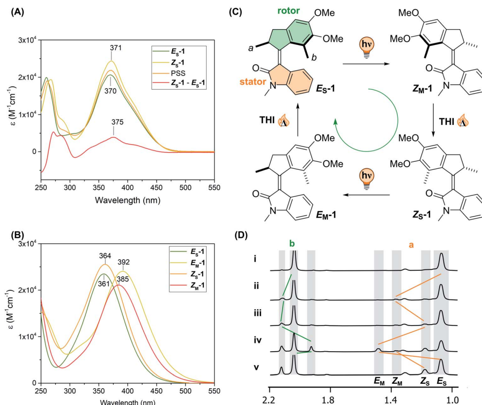
Fig. 2 (A) Steady-state UV-Vis spectra of a 3.8 × 10 -5 M methanol solution of Z S - 1 (yellow), E S - 1 (green) – and their difference (red) and photostationary state (PSS, orange) obtained upon 365 nm illumination for two minutes at room temperature. (B) Simulated absorption spectra and their maxima calculated at the PCM(MeOH)-TD-ωB97X-D/6-311+G(2d,p)//PCM(MeOH)-MP2/6-31G* level of theory for E S - 1 , E M - 1 , Z S - 1 and Z M - 1 . (C) Rotation cycle of motor 1 . (D) Selected parts of 1 H NMR spectra of E S - 1 in CD 2 Cl 2 (3.8 × 10 -3 M) (i) E S - 1 before irradiation; (ii) after 30 min irradiation at 365 nm at –90 °C; (iii) no irradiation, THI, –90 °C, 10 min; (iv) after additional 104 min irradiation at 365 nm at –90 °C (PSS 365 nm); (v) no irradiation, THI, –45 °C, 15 min.
