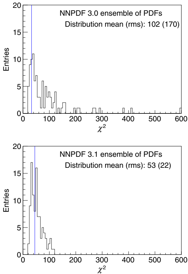
FIG. 23. Distribution of \chi^2 values from the comparisons between the measurement and the individual predictions over 15 bins for the NNPDF 3.0 and NNPDF 3.1 ensembles of PDFs. The light (blue) vertical line of each panel show the \chi^2 value of the ensemble-averaged prediction for NNPDF 3.0 (32.6) and NNPDF 3.1 (44.9). For NNPDF 3.0, one of the ensemble PDFs gives a \chi^2 value of 1548, and is not shown. For NNPDF 3.1, all values are contained within the panel.
