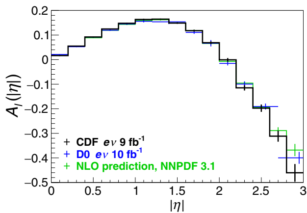
FIG. 20. Distributions of A_e(|\eta|) as a function of |\eta| for the Tevatron measurements previously shown in Fig. 19, along with the NLO prediction with NNPDF 3.1 PDFs. The bold (black) histogram is the result of this measurement and the (blue) crosses the D0 measurement [8]. The thin (green) histogram is the NLO prediction using the NNPDF 3.1 PDFs.
