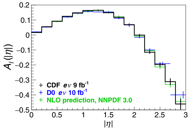
FIG. 19. CP-folded distributions of A_e(|\eta|) as a function of |\eta| . The bold (black) histogram is the result of this measurement, and the uncertainties shown are evaluated bin-by-bin and include both statistical and systematic contributions. The (blue) crosses represent the measurement from D0 [8]. For D0, the bin size is also 0.2 |\eta| -units wide, except for these regions: 1.2–1.6, 2.4–2.7, and 2.7–3.2. Both the CDF and D0 measurements use all the data from Run II of the Tevatron Collider. The thin (green) histogram is the NLO prediction using the NNPDF 3.0 PDFs.
