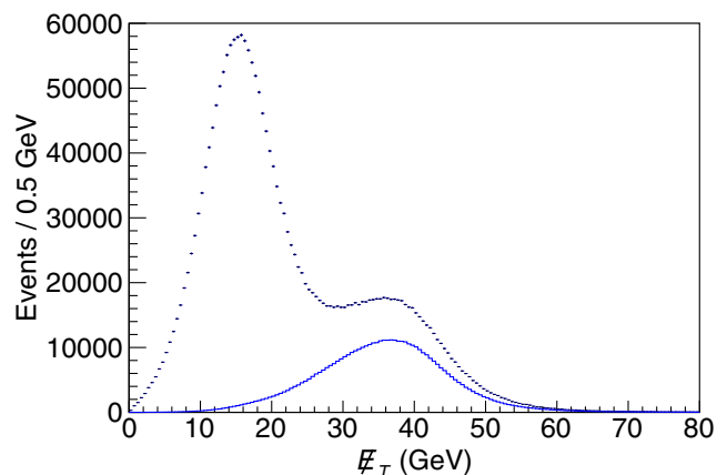
FIG. 25. \cancel{E}_T distribution for plug-region electrons rejected by the additional selection criteria. The (black) crosses are the data, and the (blue) histogram is the simulation, which contains about 18% of the events without the additional requirements. The online-trigger selection allows the peak at low values of \cancel{E}_T .
