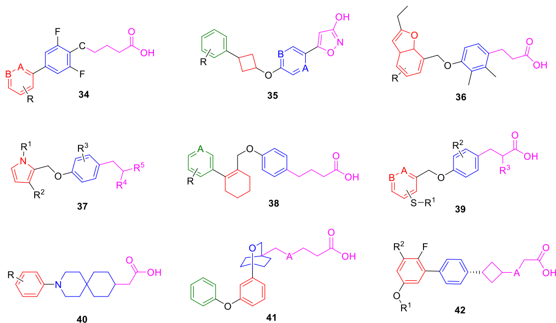
Figure 8. Patented general chemical structure useful GPR120 agonists.
