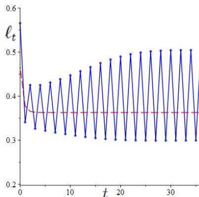
Figure 4. Parameter set: A = 10.6 , \alpha = 0.3 , \beta = .89 , \gamma = 0.64 , \delta = 0.14 and \theta = 0.2 . Time series of two distinct trajectories of \ell_t : one approaches the stationary state (red-dashed),
