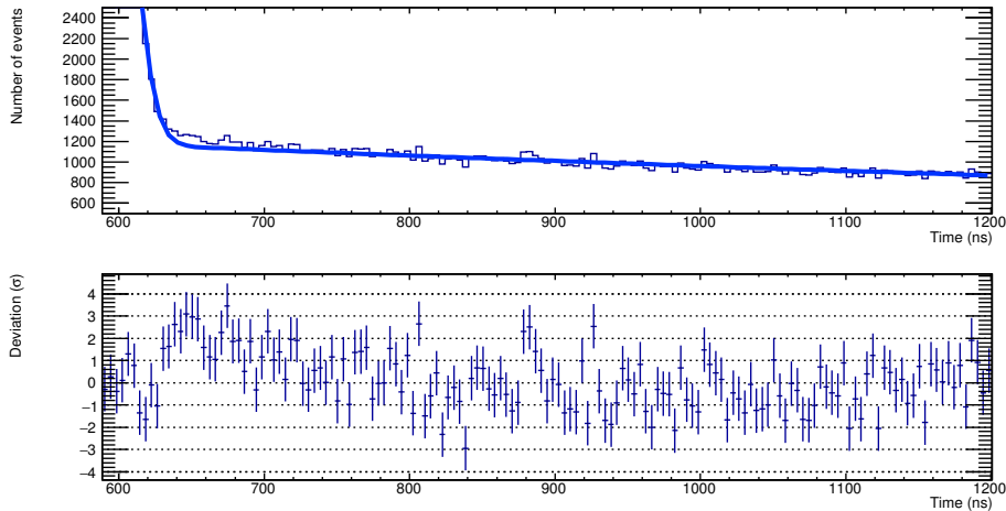
Figure 12. Top panel: fit of the time distribution for the graphite target, close up of the region after the second pulse. Bottom panel: deviation of the data from the fit ( \sigma ) in the same time region.
