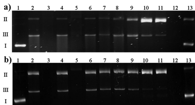
Fig. 8 Comparison of interaction of uncomplexed Cu(II) ions (even lanes) and the Cu(II)–viomycin (odd lanes) on plasmid DNA in the presence of H_2O_2 (a) 50 \mu M , (b) 25 \mu M . Lane 1, plasmid; lane 2, plasmid + 500 \mu M Cu(II) + H_2O_2 ; lane 3, plasmid + 500 \mu M complex + H_2O_2 ; lane 4, plasmid + 250 \mu M Cu(II) + H_2O_2 ; lane 5, plasmid + 250 \mu M complex + H_2O_2 ; lane 6, plasmid + 100 \mu M Cu(II) + H_2O_2 ; lane 7, plasmid + 100 \mu M complex + H_2O_2 ; lane 8, plasmid + 50 \mu M Cu(II) + H_2O_2 ; lane 9, plasmid + 50 \mu M complex + H_2O_2 ; lane 10, plasmid + 10 \mu M Cu(II) + H_2O_2 ; lane 11, plasmid + 10 \mu M complex + H_2O_2 ; lane 12, plasmid + 500 \mu M viomycin + H_2O_2 ; lane 13, plasmid + 10 \mu M viomycin + H_2O_2 .
