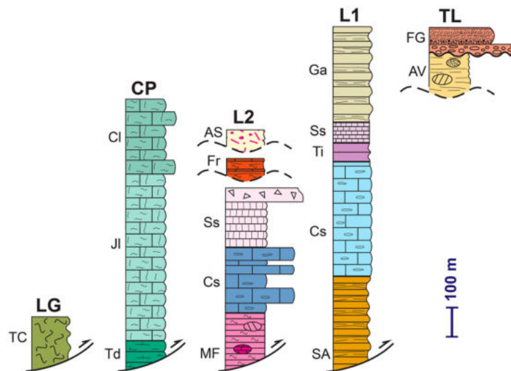
Figure 2. Stratigraphic sections from the study area (after Bucci et al., 2012, modified). AV, Argille Variegata group (late Cretaceous to Oligocene); AS, Argilliti del Torrente Serrapotamo (Oligocene); Cl, Cretaceous limestone; Cs, Calcari Con Selce Formation (Late Triassic); Fr, Flysch rosso formations (late Cretaceous to Oligocene); FG, Flysch di Gorgoglione (middle Miocene); Ga, Flysch Galestrino (Cretaceous); JI, Jurassic limestone; MF, Monte Facito Formation (Middle to Late Triassic); SA, Sorgente dell'Acero formation (Carnian); Ss, Scisti silicei (Jurassic); TC, Torrente Cavolo formation; Td, Triassic dolostone; Ti, Intervallo di transizione (late Norian to Rhaetian).
