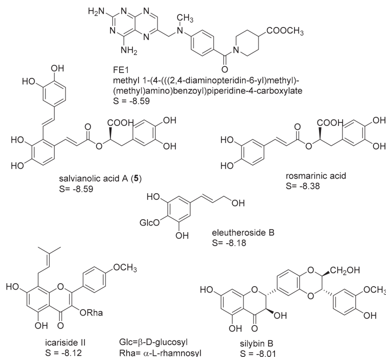
Figure 3. Best five hits from the virtual screening based on the FE1 pharmacophore ( LmPTR1 PDB-ID "2QHX"); S-scores of the induced-fit docking simulations are given in kcal/mol. A "self-docking" computation of the co-crystallized inhibitor FE1 was performed accordingly.
