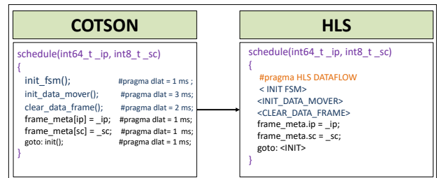
Fig. 1: Translation of the schedule function from COTSon simulator to Xilinx Vivado HLS tool in a nutshell.
