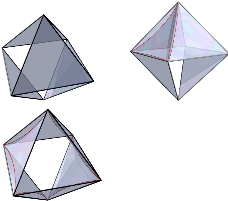
Figure 6: Three examples of non-simply connected minimal films spanning the boundary of a regular octahedron. Top-left: trivial nonconnected surface consisting in four of the eight faces; Top-right: surface obtained by starting from five of the eight faces, the result consists in an isolated triangular face F (after removing its boundary) plus a film with three triple curves wetting all the edges of the octahedron that are not edges of F ; Bottom: surface obtained by starting from six of the eight faces. Note the presence of six triple curves. Images obtained using the surf code by E. Paolini.
