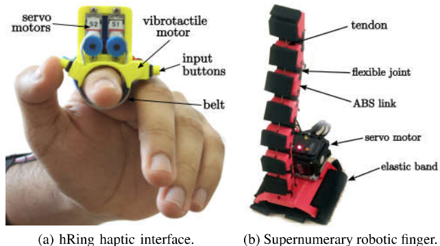
Fig. 2. The hRing and the supernumerary robotic finger.
