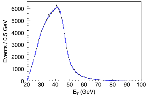
FIG. 15. E_T distribution for the CP -topology electron with the larger E_T . The crosses are the background-subtracted data, and the solid histogram is the simulation.
