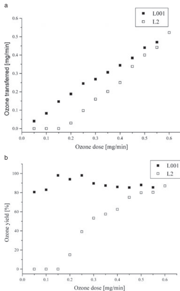
FIG. 2. (a) Transfer and (b) total yield of ozone obtained by using ozone generator A and two different GED's sizes.
