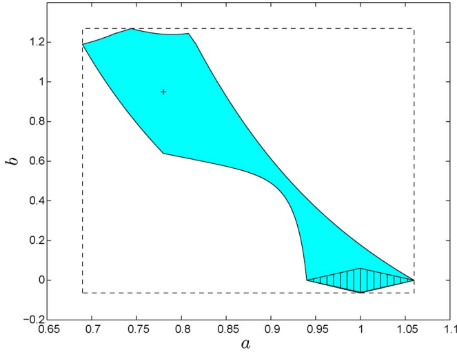
Fig. 4. Example 1. Feasible set (filled region), set \mathcal{I} (striped region) and computed outer box. The true parameter vector is marked by a cross.
