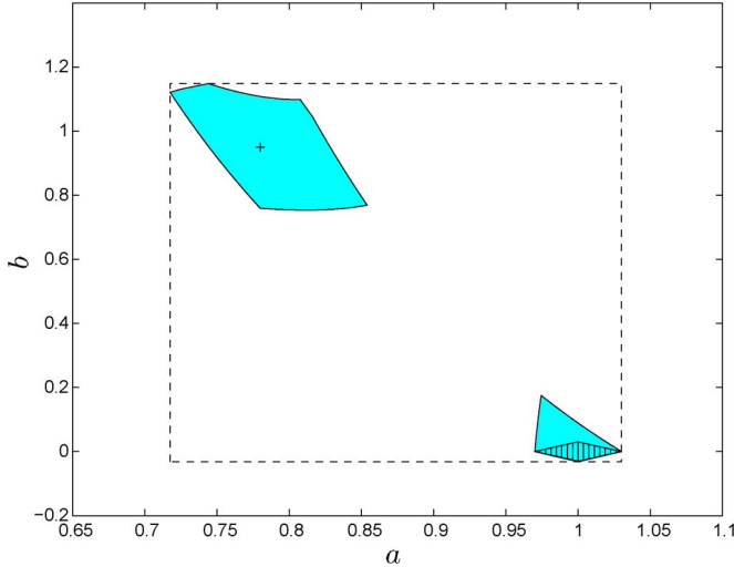
Fig. 5. Example 1. Feasible set (filled region), set \mathcal{I} (striped region) and computed outer box. The true parameter vector is marked by a cross.
