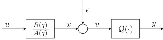
Fig. 2. Structure of the OE model with quantized measurements.
