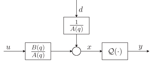
Fig. 3. Structure of the ARX model with quantized measurements.
