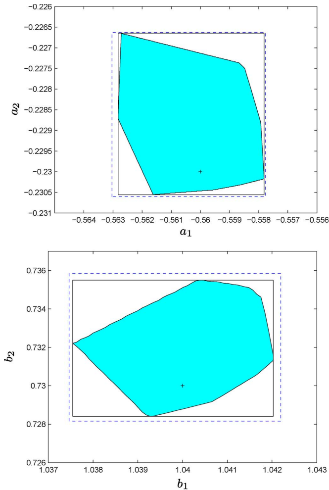
Fig. 7. Example 2. Sets \mathcal{F}_a (top) and \mathcal{F}_b (bottom), true parameter value (cross), minimum outer orthotope (solid) and computed outer orthotope (dashed).
