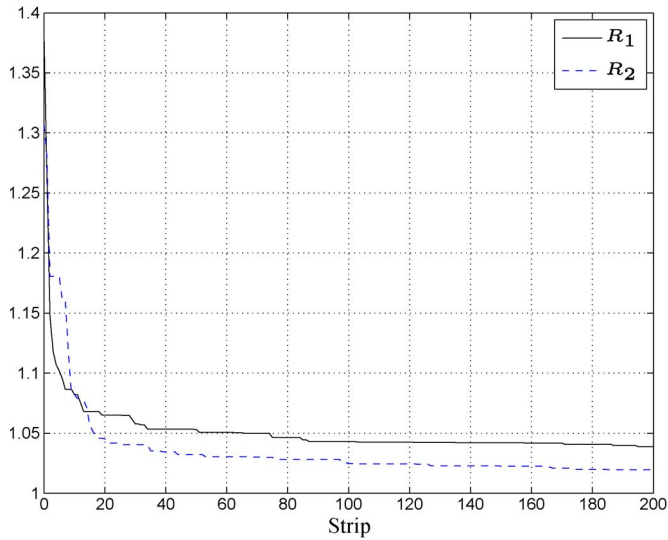
Fig. 9. Example 5. Indexes R_1 and R_2 against the number of approximating strips.
