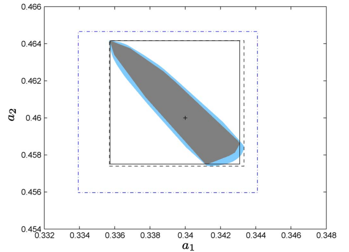
Fig. 8. Example 5. True feasible set (dark) and its polytopic approximation (light) on parameters a_1, a_2 . Boxes denote the minimum outer orthotope (solid), final outer orthotope (dashed) and outer orthotope obtained by the procedure of Section III (dashed-dotted).
