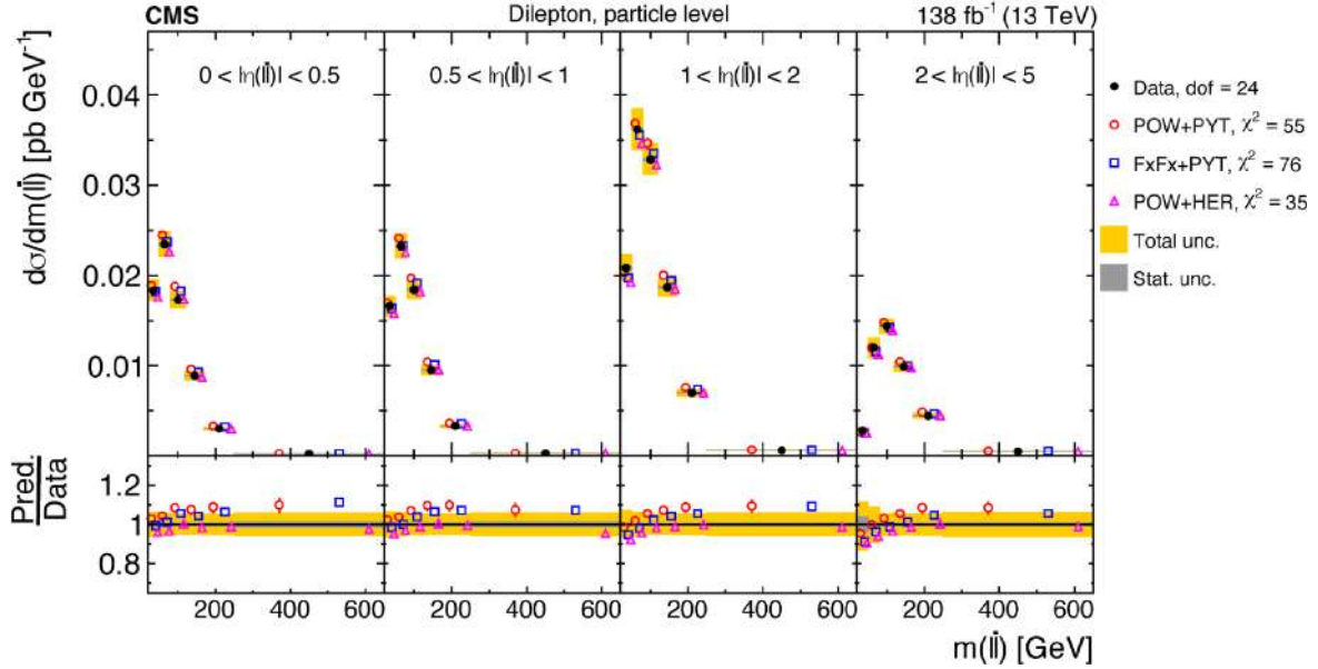
Figure 86. Absolute [\eta(\ell\bar{\ell})] cross sections are shown for data (filled circles) and various MC predictions (other points). Further details can be found in the caption of figure 82.
