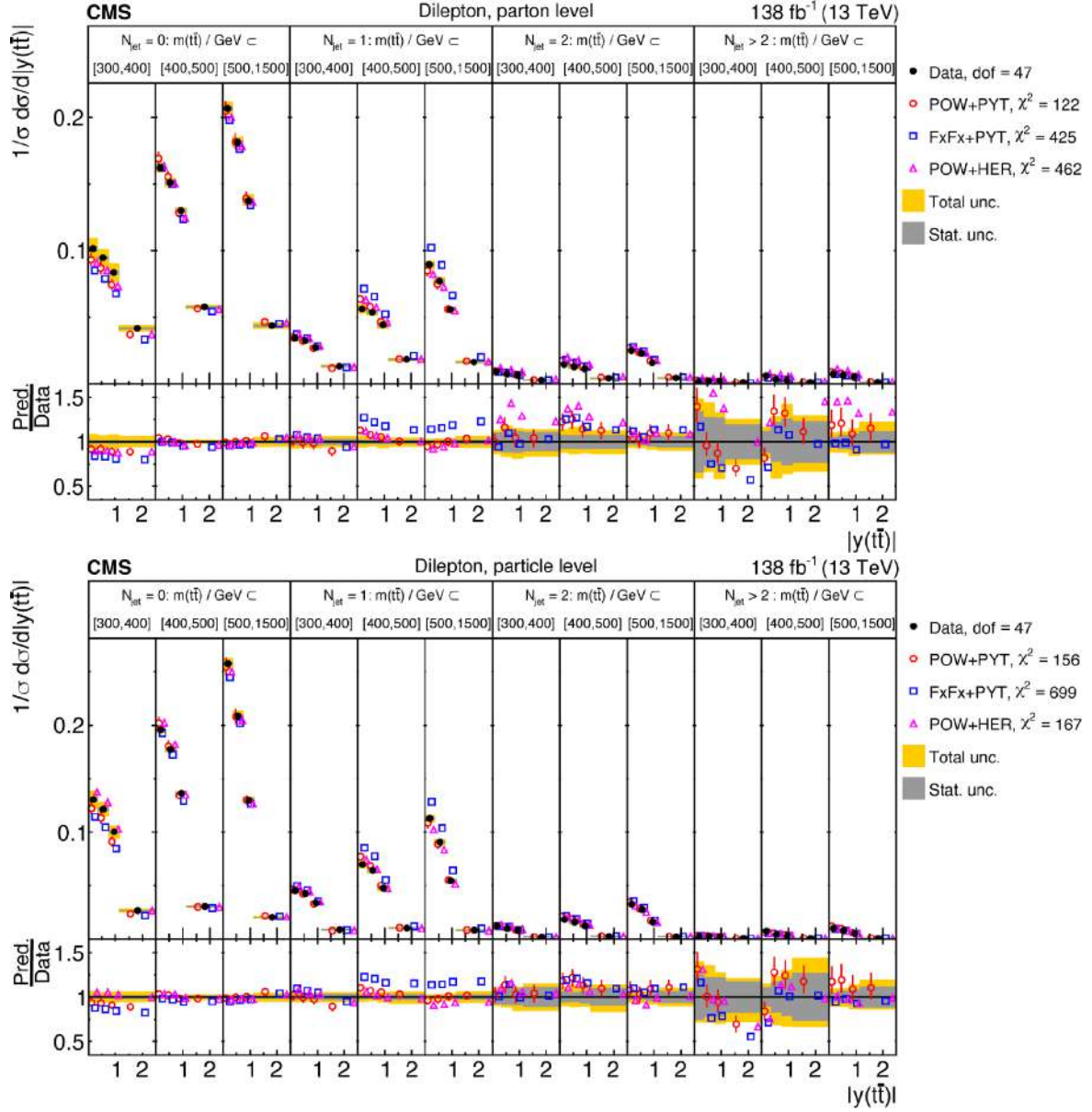
Figure 40. Normalized [N_{\text{jet}}^{0,1,2,3+}, m(t\bar{t}), |y(t\bar{t})|] cross sections are shown for data (filled circles) and various MC predictions (other points). Further details can be found in the caption of figure 32.
