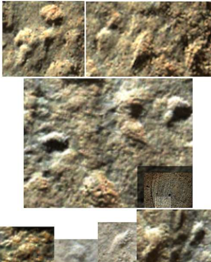
Figure 32. Sol 0553. An assemblage of fossils like forms ranging from 1-5 mm in size as also depicted in Figure 31.
