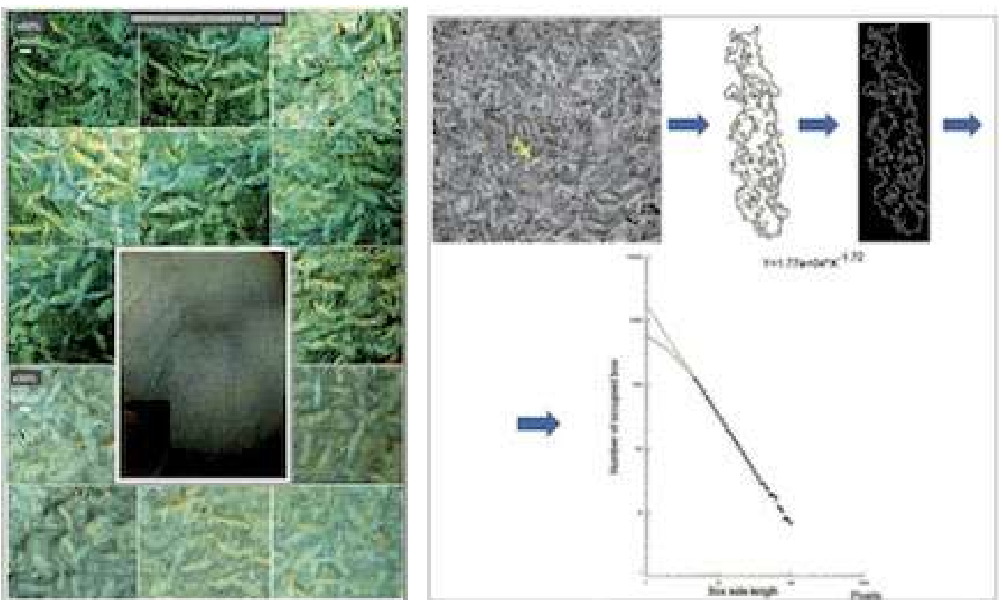
Figure 20. Sol 809 depicting elongated fusiform shaped formations. A canny filter was used to create negative images for the purpose of fractal analysis (Rizzo, et al. 2021). The log plot is a strength line (p, 0.01) indicating that the vast majority of these light-colored elongated structures have a fractal structure of self-similarity; its exponent the fractal dimension. These findings are compatible with biology, but not crystallization.
