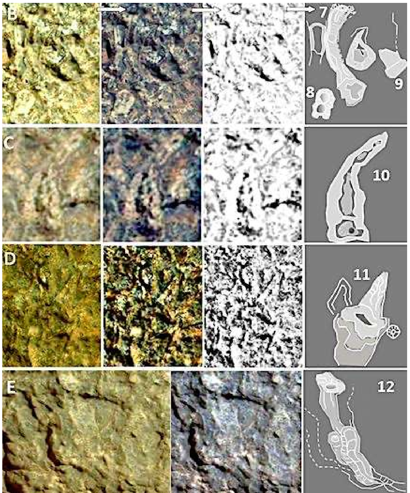
Figure 41. Microanalysis of Sol 553. B-E are also identified in Figure 41 and include paint-net processing with black and white highlighting of the most salient features. 7-9 reveals forms that are hollow, branched, fusel structure, and 7 with an internal cavity that widens towards the two ends whereas. in 10 one end is narrow the other wide. 8 includes structures with two smooth lobes side by side and joined together by a clear, knurled frame, which together constitute a single and distinct structure. 10 has a conical and curved shape with a central cavity rising irregularly upwards with walls forming a radial system at the top. In box D a clear conical shape which becomes enlarged in a shapeless flaring and which may overlap with another structure In box E irregular conical shapes include those that are hollow and with set walls, some of which develop within a branched system starting from a vertex (bottom). 3 is suggestive of microspheres and laminae that wrap either in a chaotic way or in a regular way, whereas in 11 they form overlapping structures with cones or tubular shapes (1,6,7,10,11,12). The overall chaotic pattern is similar to what might be expected of numerous organisms that were oriented differently when fossilized.
