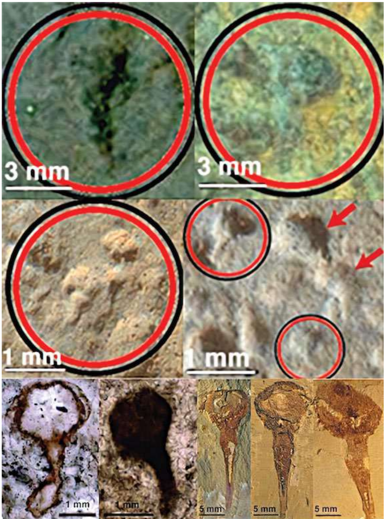
Figure 11. (First row): Sol 809 and Sol 869. (Second row) Sol 905 and Sol 905. Specimens photographed in Gale Crater and that are quantitatively and statistically significantly similar to Ediacaran fossils of Namacalathus (Earth, Bottom Row) Cambrian fossils of Lophotrochozoa (three bottom right). Photos of Namacalathus reproduced from and courtesy of Kontorovich A E, et al. [42]. Photos of Lophotrochozoa reproduced from and courtesy of Zhang ZF, et al. [43]
