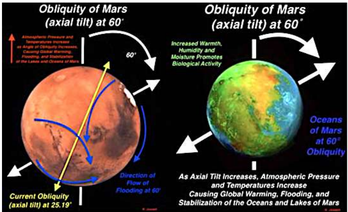
Figure 43. The obliquity of Mars can range up to 82 degrees.
