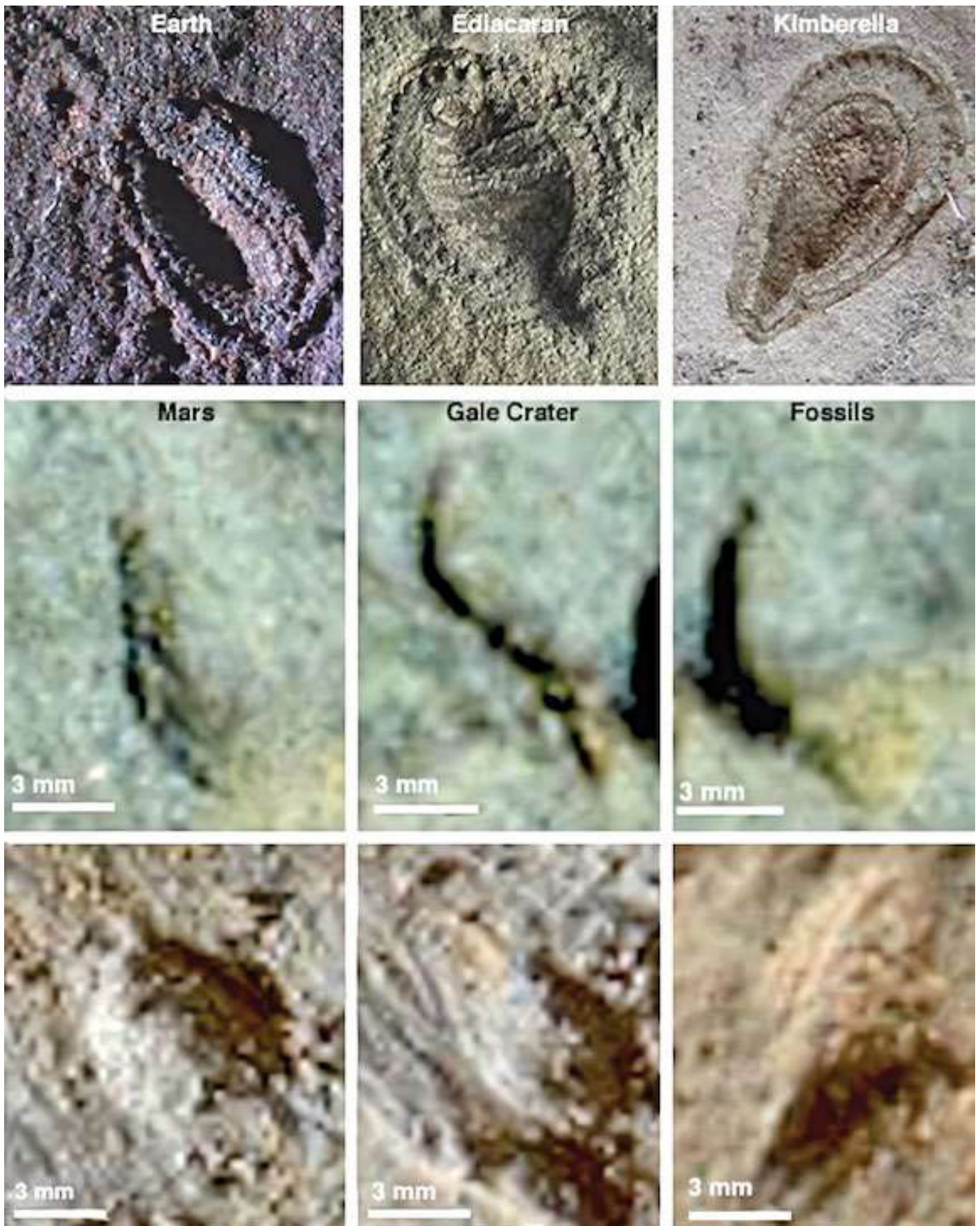
Figure 12. Earth (First row) fossilized remains of Ediacaran Kimberella. (Mars, Bottom two rows): Specimens photographed in Gale Crater, quantitatively and statistically indistinguishable from Ediacaran fossils of Kimberella . Sol 809, Sol 809, Sol 809; Sol 880, Sol 905, Sol 905. Note proboscis and pleopod appendages.
