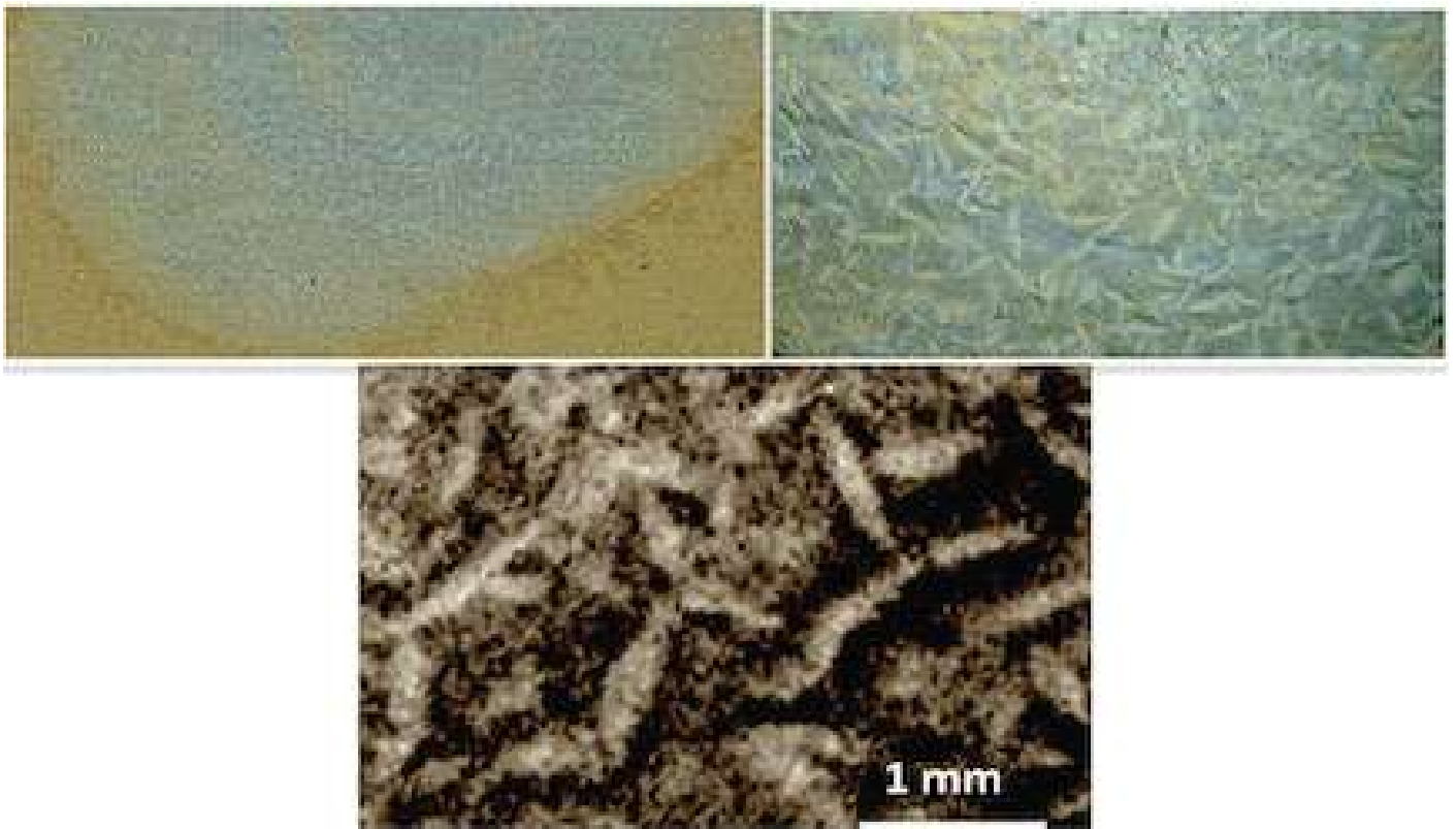
Figure 19. Sol 809: (Bottom enlarged, desaturated). These specimens resemble mineralized trace fossils possibly created by colonies of unknown organisms that may have been mineralized. The orientation of the spindle-like, whitish structures are not organized like mineral structures. Quantitative morphological analysis by Rizzo et al. (2021) supports the hypothesis that these may be biological in origin.
