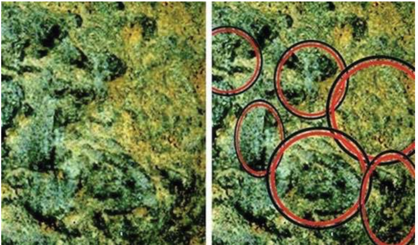
Figure 10. Sol 0809. An assemblage of fossils like forms ranging from 1-5 mm in size.
