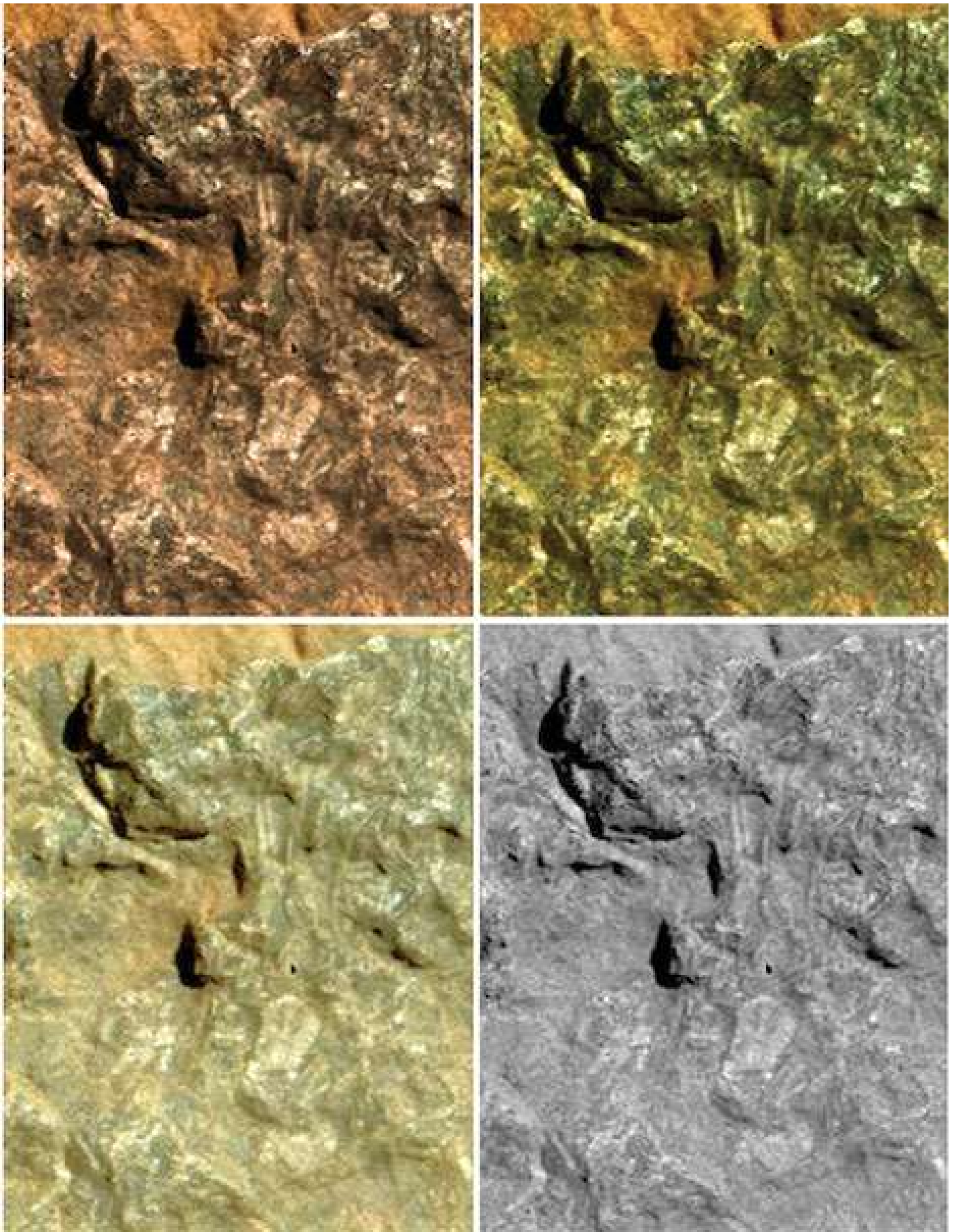
Figure 6. Sol 0553. Magnified color saturated/desaturated section of Figure 1. An assemblage of fossils?.
