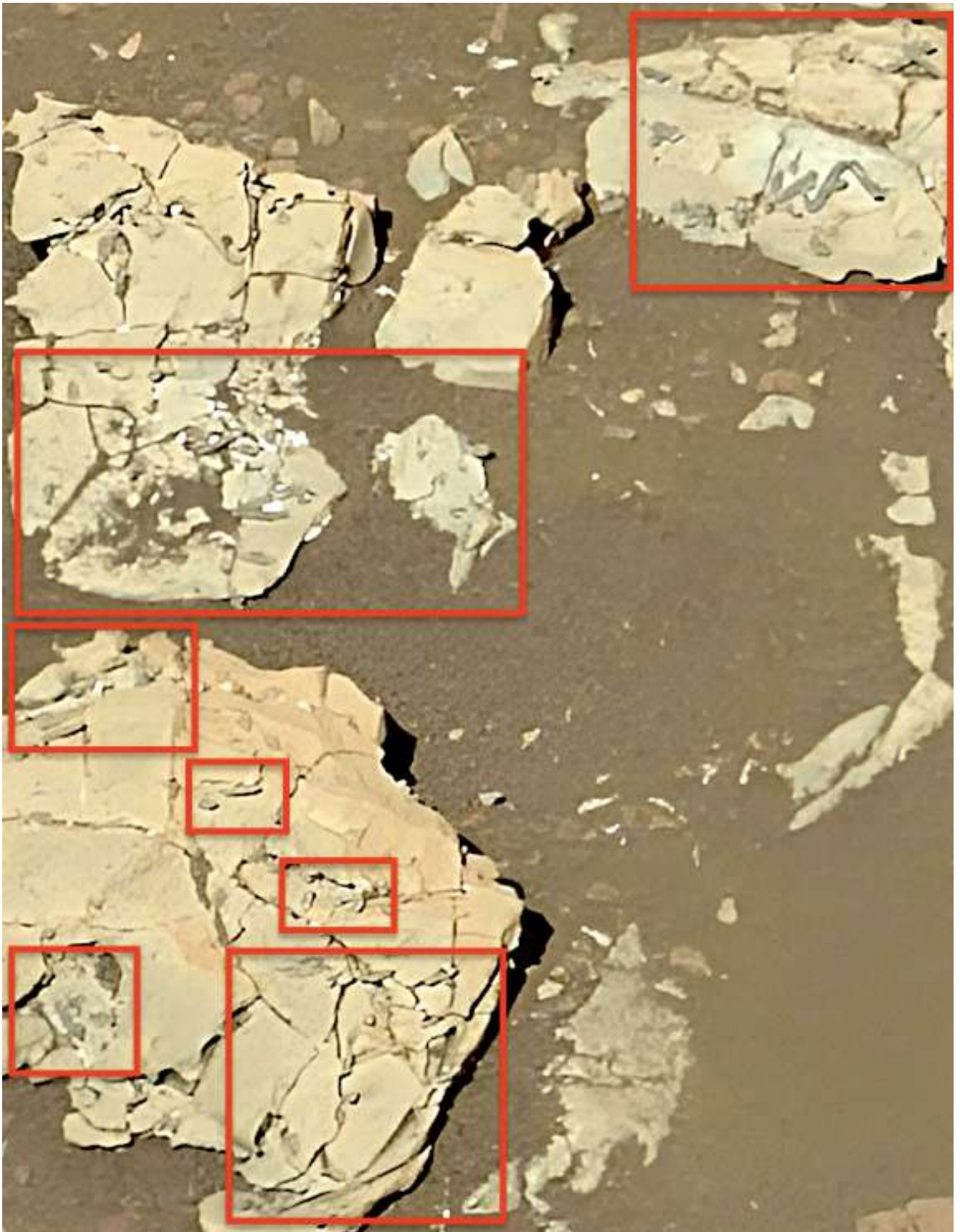
Figure 37. Sol 1921. Numerous tubular formations laying upon different rocks. Supporting the hypothesis these were living organisms, the tableau vivant is compatible with mineralization following the rapid receding of the waters. 1921MR0100290000900414E01_DXXX.
