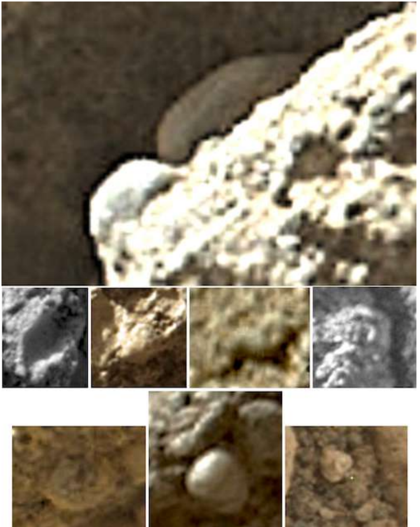
Figure 34. A variety of worm-like forms photographed on Sol 1032. MH0005070010400164C00_DXXX.
