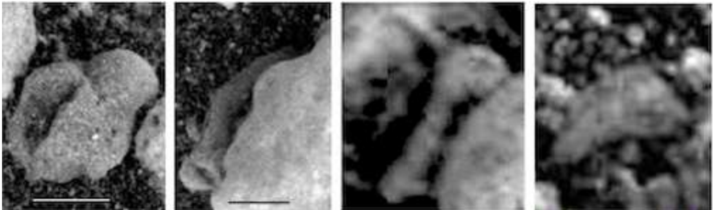
Figure 39. Endurance Crater. Tubular forms photographed in an ancient lake bottom adjacent to holes in the ground that may have been thermal vents [14]. 1M145852648EFF3505P2957M2M1.
