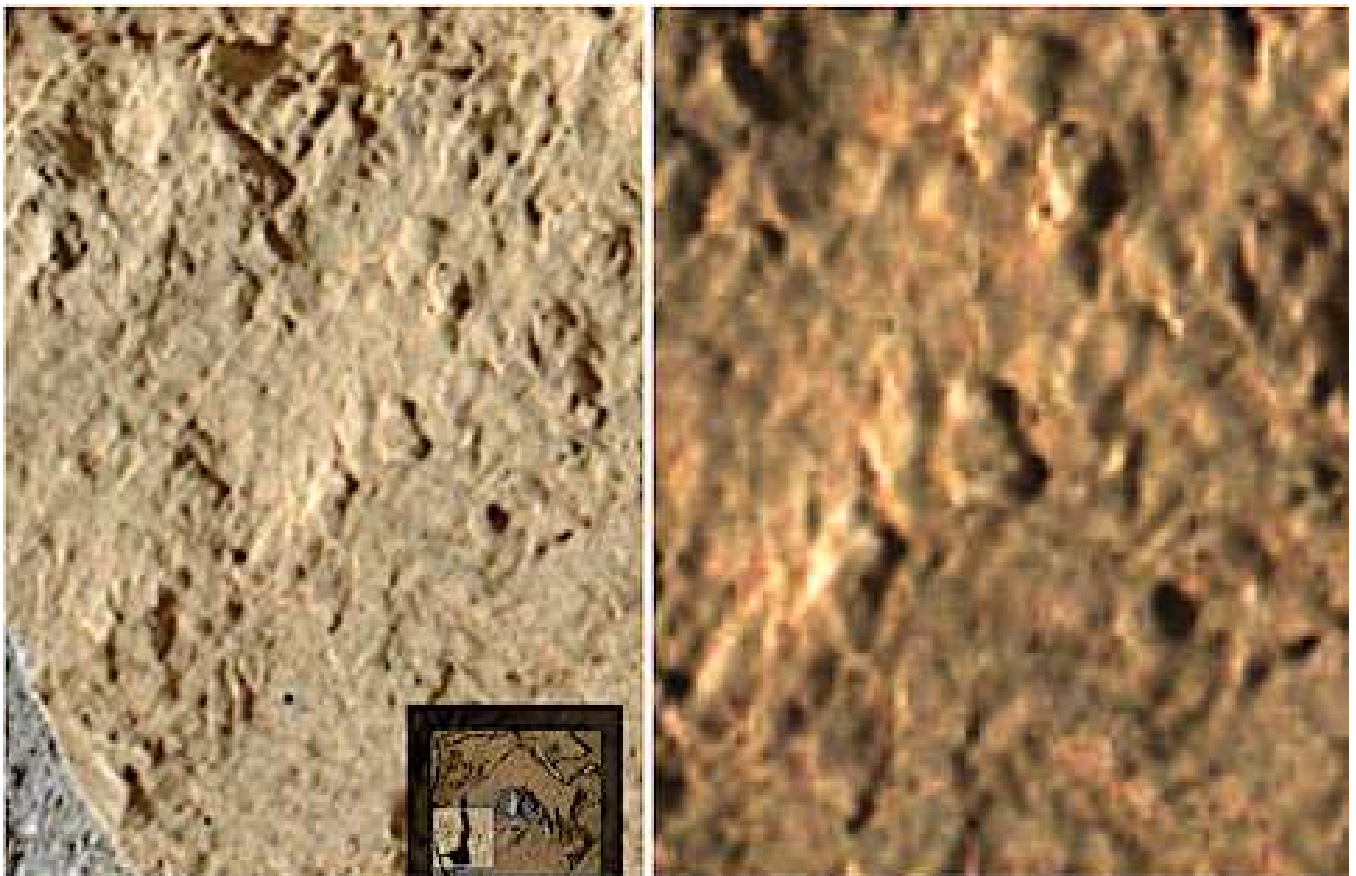
Figure 25. Sol 869. Fossil-like specimens resembling a variety of organisms. 0869MH0002650000302304R00_DXXX.
