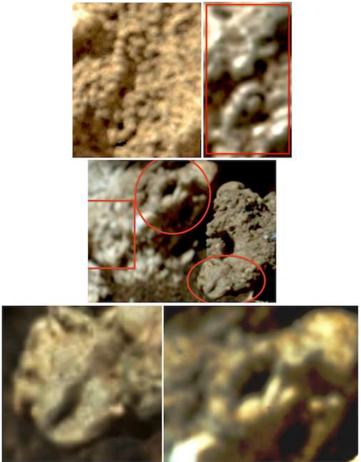
Figure 35. Worm-like forms photographed on Sol 1032. MH0005070010400164C00_DXXX.
