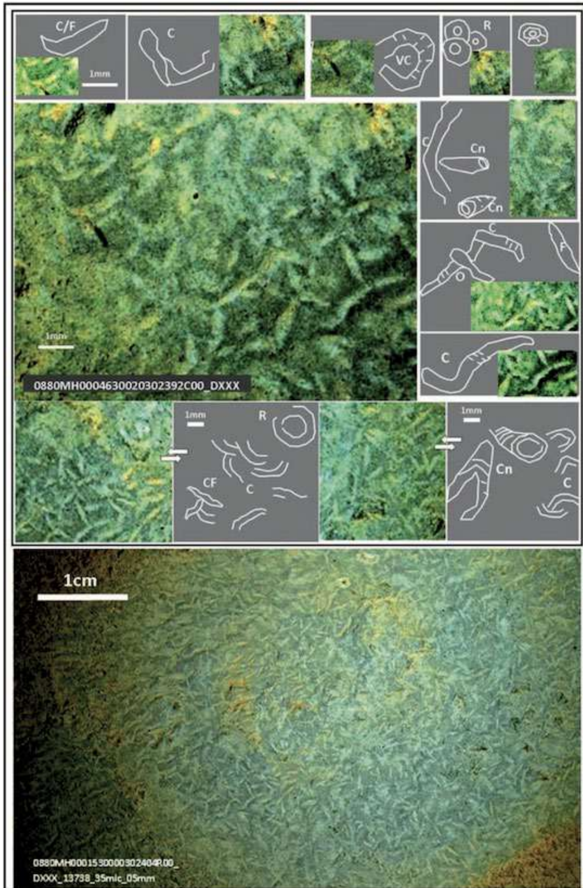
Figure 21. Sol 809, 880. Morphological analysis of the elongated and globular light colored specimens depicted in Sol 809 and Sol 880. It is evident there are repetitive (C), overlapping (O), conical (Cn) very curved (VC) ring-shaped (R) curved fusiform (C/F) shapes. These patterns and shapes are not what would be expected if these were embedded crystals (Rizzo et al. 2021). Compare with Figure 21.
