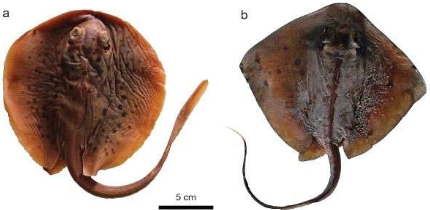
Figure 30. a) Taeniura lymma ; b) Neotrygon sp. From a collection at the Institute of Paleontology of the University of Vienna. CREDIT: Giuseppe Marrama.
