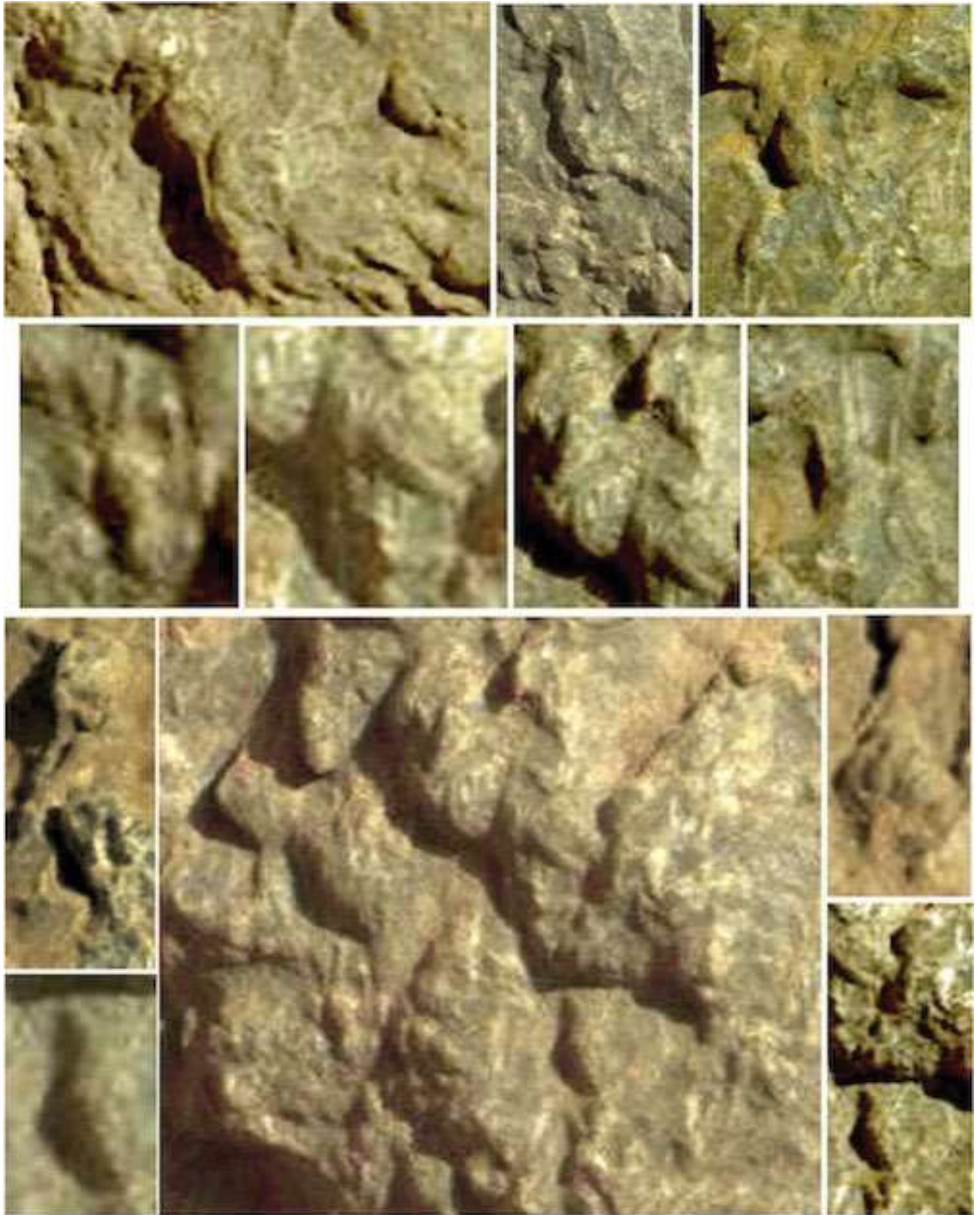
Figure 4. Sol 0553. Magnified section of Figure 1. An assemblage of fossils like forms ranging from 1-5 mm in size.
