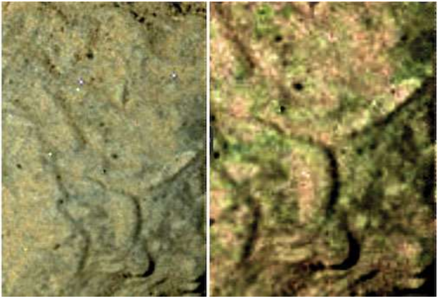
Figure 24. Sol 869. worm-like specimens embedded atop mudstone/sandstone. Approximately 1-3 mm in length. 869MH0004600020302294C00_DXXX.
