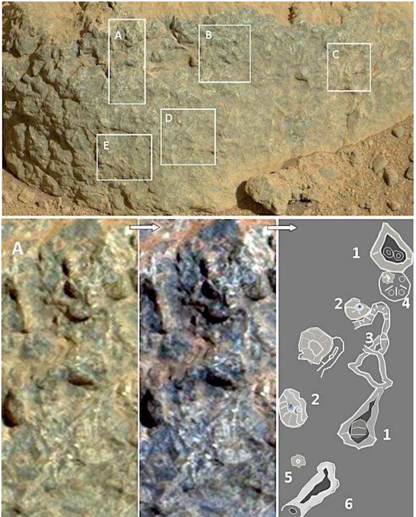
Figure 40. Microanalysis analysis of Sol 553, sharpened and amplified via Paint net. Chaotic microstructures, similar to possible microfossils are evident as based on their istinct shapes as defined by color, roughness and relief, elevation, which indicate individuality including those that are 1 conical, 2 rolled, 3 elongated and overlapping, 4 globular, 5 tubular and possibly hollow. These individual forms are distinct from the underlying sediment which may be a fragment of a coral reef. Additional micro-analysis of Sol 552 is presented in Figure 41.
