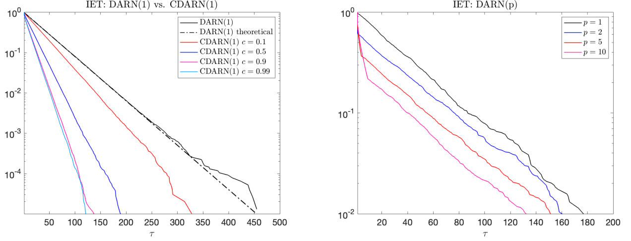
FIG. 12. Comparison of the Inter-Event Time (IET) distributions between DARN(1) and CDARN(1) (LCC) models (left), and of the DARN(p) models for different p (right). IET is obtained by using simulations of time series of length T = 10^5 of the models, with y = 0.1 , q = 0.75 , and c as indicated in the plots (for CDARN).
