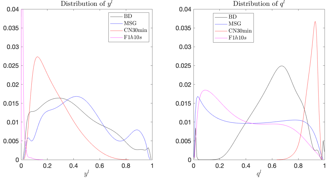
FIG. 5. Distribution of y^\ell (left) and q^\ell (right) of the heterogeneous CDARN(1) (LCC) model estimated on temporal network data built for four datasets as indicated in the legend. Parameters are estimated by solving Eqs. (92) and (93), respectively.
