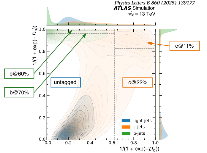
Fig. 2. Distribution of light, c -, and b -jets for the 2D b/c -tagger in simulated t\bar{t} events. Dashed lines correspond to the edges of the working points. For visualization purposes a standard logistic function is applied to both axes of the discriminant. The contours for each jet type are smoothed with a kernel density method to improve readability, with contours corresponding to lines of constant density. The two b -tagging bins comprise the top left corner of the discriminant, with the c -tagging bins to the right of the vertical dashed line. Untagged jets are located in the bottom left corner.
