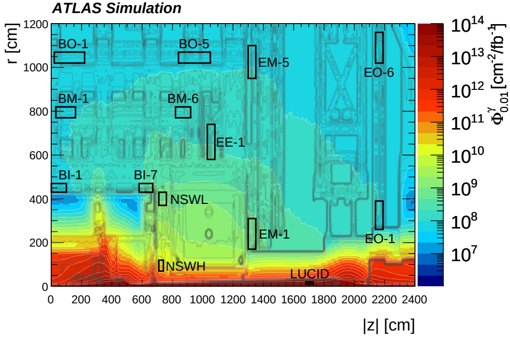
Figure 15. Contours of constant fluence for photons with E > 10 keV ( \Phi_{0.01}^{\gamma} ) in the ATLAS cavern and muon spectrometer regions. The black boxes indicate regions over which the main radiation quantities given in table 7 are averaged. More detailed explanations of the detectors in these regions can be found in section 5. The faint grey lines are density contours from the GEANT4 geometry model and only serve to give an indication of the detector geometry.
