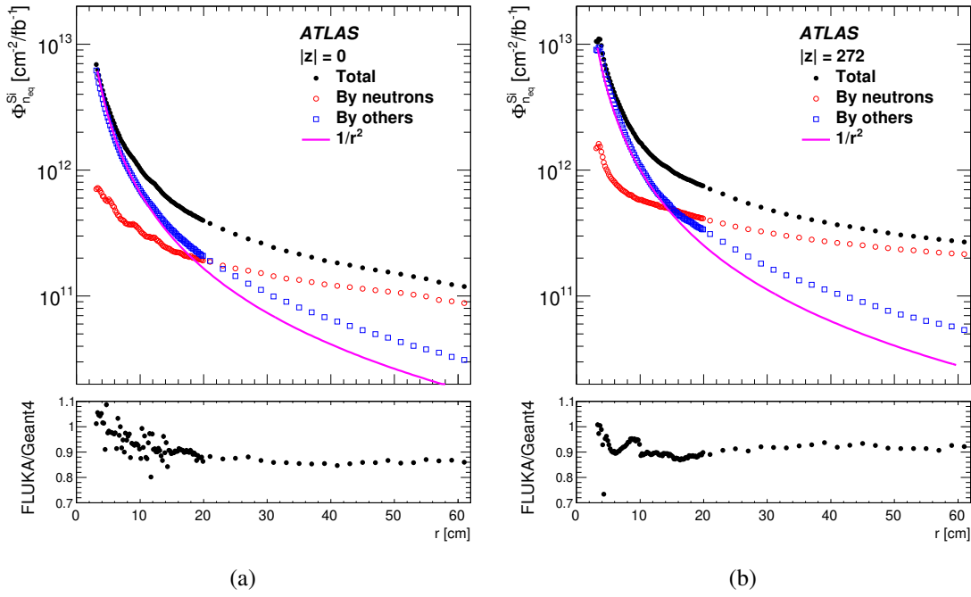
Figure 12. Radial dependence of \Phi_{n_{eq}}^{\text{Si}} at (a) |z| = 0 and (b) |z| = 272 cm in the ID , as obtained from FLUKA simulations. The total \Phi_{n_{eq}}^{\text{Si}} is divided into the contribution by neutrons and by all other particles. The r^{-2} dependence is normalised at r = 3.1 cm to the ‘By others’ value. The lower panels show the ratio of FLUKA and GEANT4 results for the total.
