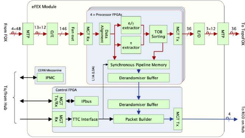
Figure 78. Block diagram of an eFEX module, illustrating the real-time and readout paths. Control and monitoring signals, except for the L1A , are not shown.
