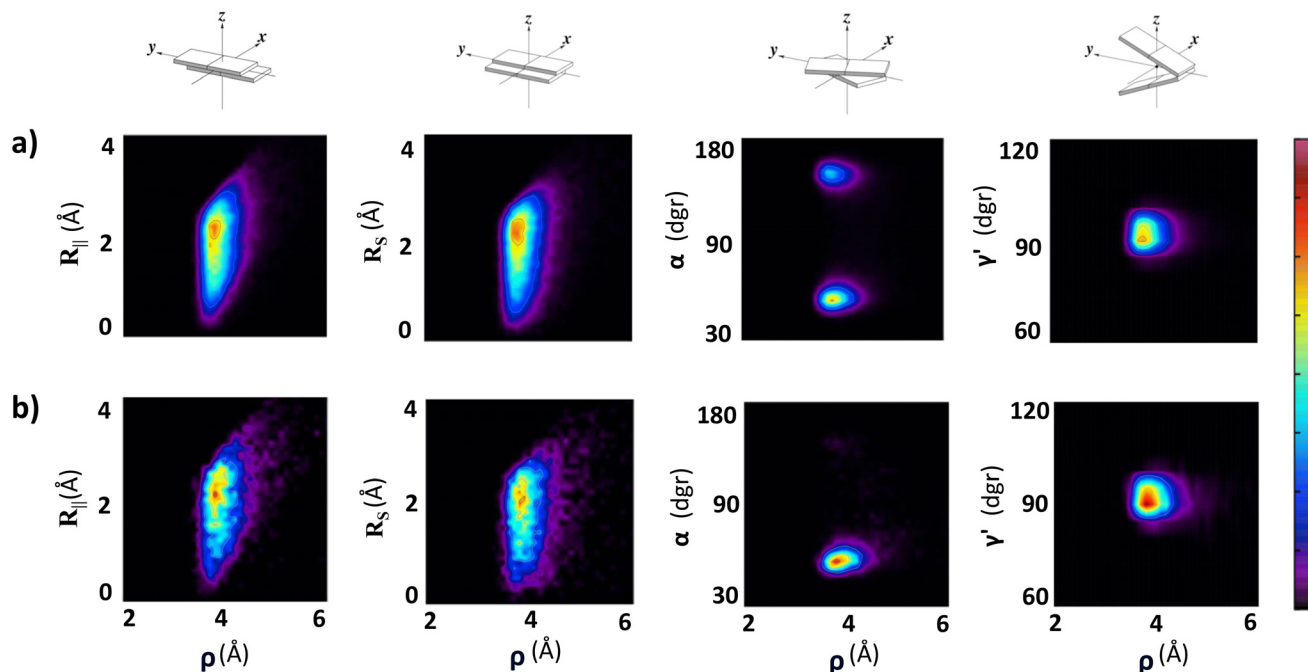
Fig. 7 2D heat maps of the distributions of the \rho distances with the geometrical descriptors defined in Fig. 2, and computed for the inner (b–c) pair along the MD trajectories produced for (a) \text{PDI}_8@H_2O , (b) \text{PDI}_{12}@H_2O . In each panel, columns refer, from left to right, to the sliding ( R_{||} ), shifting ( R_{\perp} ), spinning ( \alpha ) and tumbling ( \gamma' ) motions. For the sake of clarity, a graphical representation of the displacement associated with each geometrical descriptor is displayed in the top panel.
