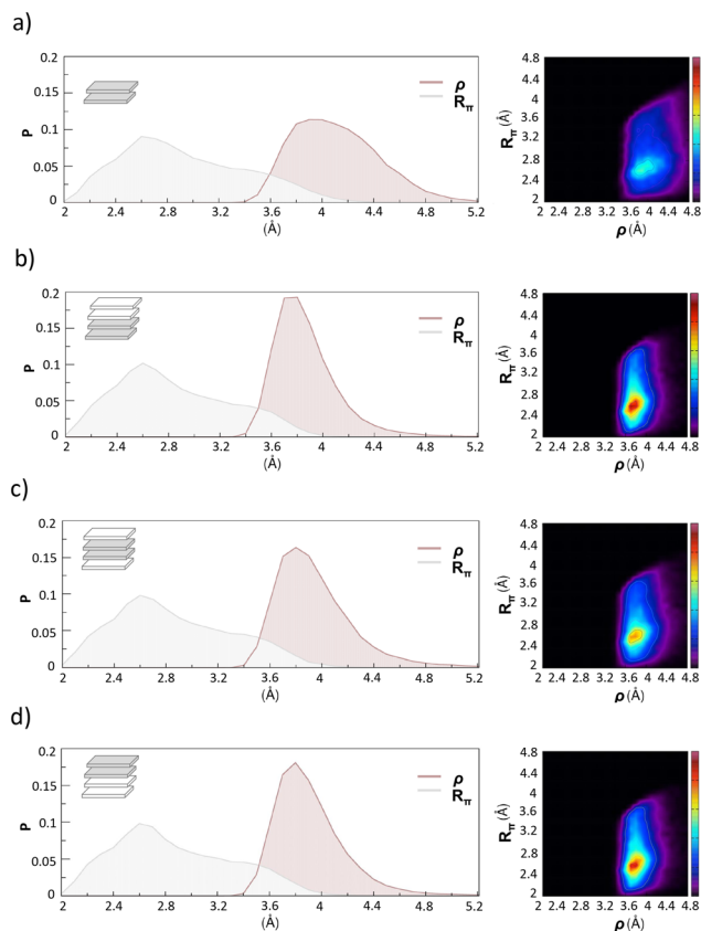
Fig. 5 Distributions (left) and 2D heat maps (right) of \rho and R^\perp (see Fig. 2 for definition), computed along either the \text{PDI}_2@H_2O and \text{PDI}_4@H_2O trajectories for (a) the \text{PDI}_2@H_2O dimer; (b) the a–b PDI pair (see inset) within the tetramer; (c) the central b–c pair; (d) the c–d pair.
