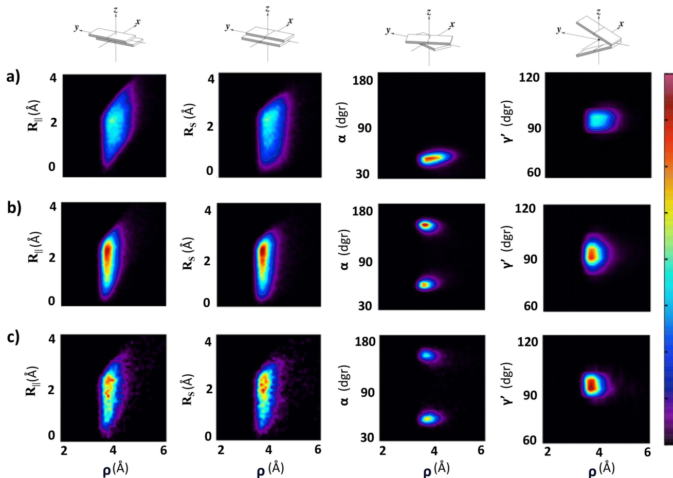
Fig. 6 2D heat maps of the distributions of the \rho distances with the geometrical descriptors defined in Fig. 2, and computed for the external (a–b) pair along the MD trajectories produced for (a) \text{PDI}_2@H_2O , (b) \text{PDI}_4@H_2O , (c) \text{PDI}_{12}@H_2O . In each panel, columns refer, from left to right, to the sliding ( R_{||} ), shifting ( R_s ), spinning ( \alpha ) and tumbling ( \gamma' ) motions. For the sake of clarity, a graphical representation of the displacement associated with each geometrical descriptor is displayed in the top panel.
