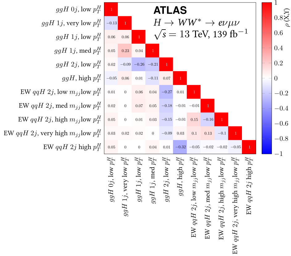
FIG. 16. Correlations between the cross-section measurements in the 11 STXS bins for the H \rightarrow WW^* \rightarrow e\nu\mu\nu analysis.
