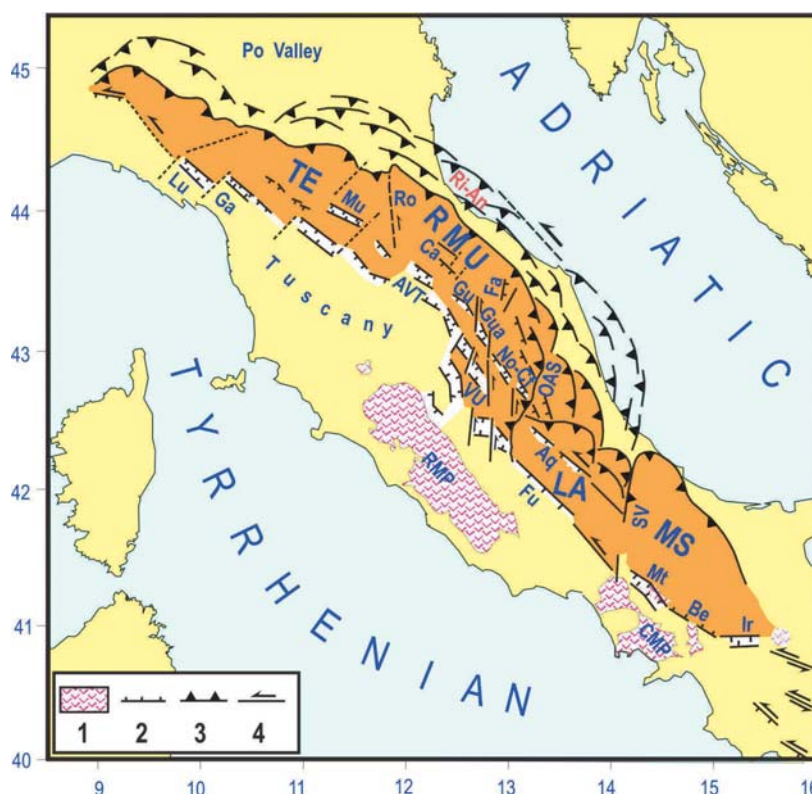
Figure 3. Tectonic setting in the Apennine belt. 1) Main Quaternary volcanic areas; 2, 3, 4) Tensional, compressional, and strike-slip features. The brown zone evidences the portion of the belt that is stressed by the Adria plate. Aq = L'Aquila fault, AVT = Alta Valtiberina trough, Be = Benevento fault, Ca = Cagli fault, CMP = Campanian magmatic province, Fa = Fabriano fault, Fu = Fucino fault, Ga = Garfagnana trough, Gua = Gualdo Tadino fault, Gu = Gubbio fault, Ir = Irpinia fault, LA = Latium-Abruzzi platform, Lu = Lunigiana trough, MS = Molise-Sannio wedge, Mt = Matese fault, Mu = Mugello trough, No-Cf = Norcia-Colfiorito fault, OAS = Olevano-Antrododo-Sibillini thrust front, Ri-An = Rimini-Ancona thrust front, RMP = Roman magmatic province, RMU Romagna-Marche-Umbria wedge, Ro = Romagna Apennines fault, SV = Sangro-Volturno thrust front, TE = Tuscany-Emilia wedge, VU = Valle Umbra fault.
