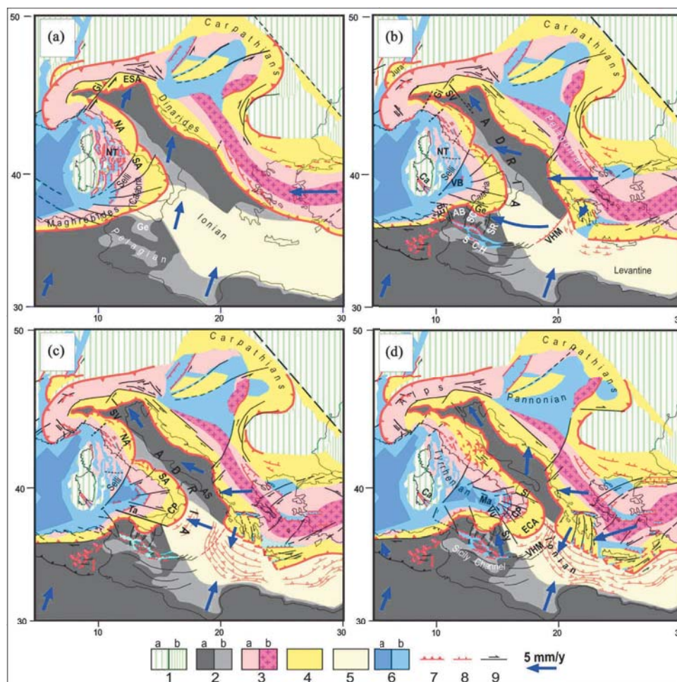
Figure 1. Proposed tectonic-kinematic evolution of the central Mediterranean region since the Miocene (e.g., [3] [5]). 1) Continental (a) and thinned continental (b) Eurasian domains; 2) Continental (a) and thinned continental (b) Nubia/Adriatic domains; 3) Anatolian-Aegean-Pelagonian belt, constituted by ophiolitic units (a) and crystalline massifs (b) 4) Other orogenic belts; 5) Ionian Tethys oceanic domains 6) Zones affected by intense (a) or moderate (b) crustal thinning; 7, 8, 9) Compressional, tensional and strike-slip features. Blue arrows indicate the proposed kinematic pattern [2]-[7]. Present geographical contours (thin black lines) are reported for reference. (a) Late Miocene. The reactivation of the Giudicarie fault system (Gi) allowed the main Adriatic domain to move roughly NE ward with respect to its northwestern edge. The consequent divergence between the main Adriatic domain and the fixed Corsica-Sardinia block induced crustal extension in the interposed sector of the Alpine-Apennine belt, forming the Northern Tyrrhenian basin (NT). ESA = Eastern Southern Alps; NA = Northern Apennines; SA = Southern Apennines; (b) Early Pliocene. The westward push of the Anatolian-Aegean-Pelagonian system causes the decoupling of the Adria plate from Nubia by the activation of the Victor Hensen-Medina-Sicily Channel fault system. Once decoupled, Adria underwent a clockwise rotation and a minor NW ward motion. The NW displacement caused the activation of the Schio-Vicenza fault system in the northern Adriatic domain. AB = Adventure block, Ca = Campidano graben, Eg = Egadi fault, Ge = Gela nappe, SCH = Sicily Channel, SC = Sciacca fault, SR = Scicli-Ragusa fault, SV = Schio-Vicenza fault, VB = Vavilov basin, VHM = Victor Hensen-Medina fault. (c) Late Pliocene-Early Pleistocene. Since the suture of the Southern Apennine consuming boundary the lateral escape of the Alpine-Apennine material has only involved the Calabria-Peloritani (CP) wedge, which has extruded roughly SE ward at the expense of the Ionian oceanic domain. Stressed by E-W compression, the southern Adriatic plate has undergone upward flexure, accelerating the formation of the Apulian Swell (AS). In this strong compressional context, the CP wedge has undergone fast uplift, bowing and fragmentation. (d) Pleistocene. The Nubia-Eurasia convergence along with the potential gravitational energy accumulated by the southern Adriatic in the previous phase triggered the northward displacement of Adria. Accretionary activity along the outer Calabrian front formed the External Calabrian Arc (ECA), while crustal extension developed in the wake of the migrating arc, forming the Marsili basin (Ma). Since the collision of the extruding CP wedge with the Adriatic continental domain, the escape trend of such wedge changed by activating new lateral guides, the Sibari (Si) and Vulcano-Syracuse (Vu-Sy) fault system.
