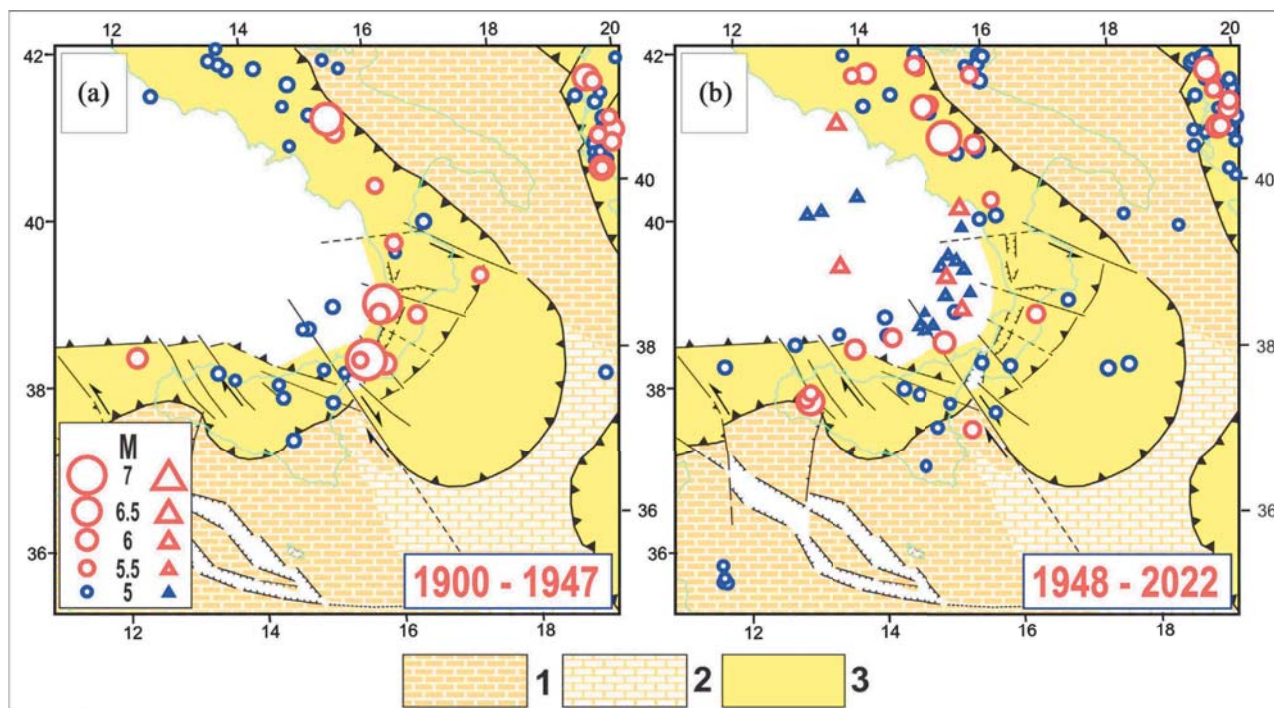
Figure 10. Seismic activity in the Sicily and Calabria zones before and after 1947. 1) Nubia-Adriatic domain 2) Oceanic Ionian domain 3) Orogenic belts. Circles and triangles respectively indicate focal depths lower and greater than 60 km. Other symbols as in Figure 5 . Seismicity data as in Figure 4 .
