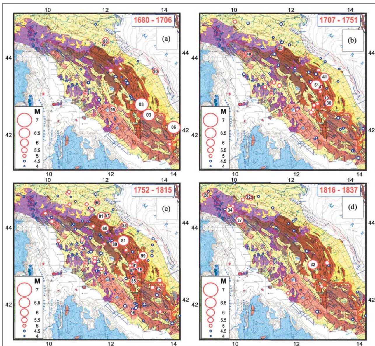
Figure 14. Distribution of the major earthquakes that followed the main 1703 shocks in the L'Aquila and Norcia faults, during the three periods considered, reported on the Tectonic Map of Italy [45]. Data from [32].
