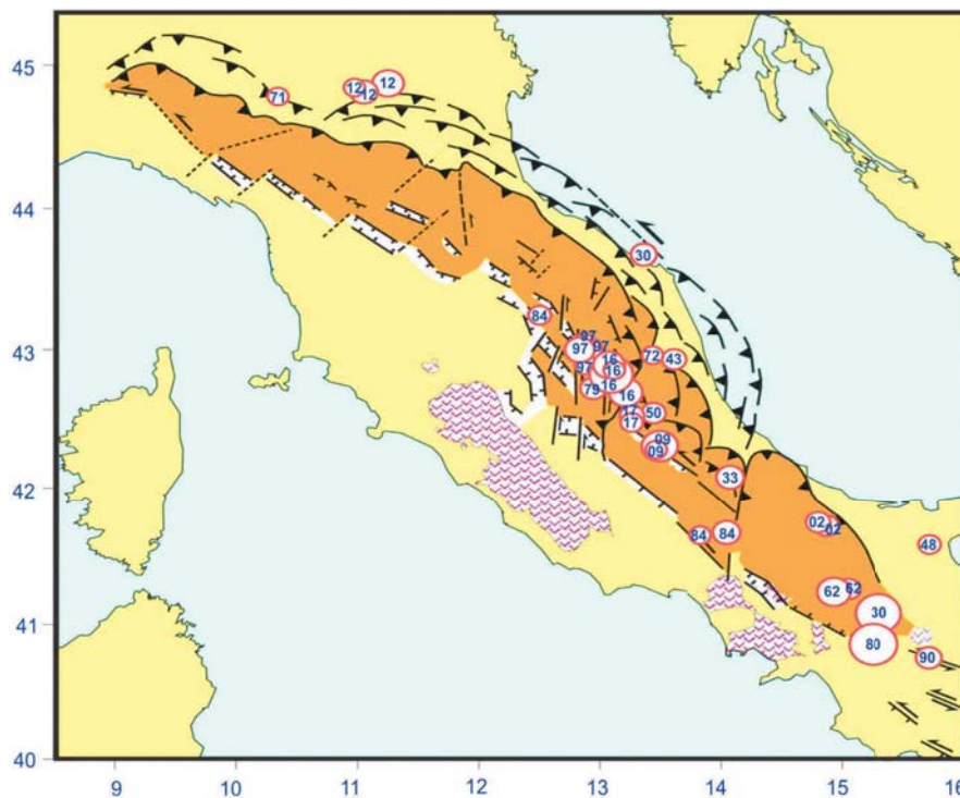
Figure 16. Main earthquakes (red circles M \geq 5.5 ) occurred since 1930 in the Apennine belt. Data from [32].
