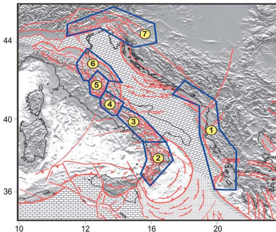
Figure 7. Geometries of the peri-Adriatic boundary zones used for studying the time patterns of seismicity ( Figure 8 and Figure 14 ). 1) Hellenides-Albanides-Southern Dinarides, 2) Calabria, 3) Southern Apennines, 4) Central Apennines, 5) Southern part of the RMU wedge, 6) Northern part of the RMU wedge, 7) Eastern Southern Alps and Northern Dinarides. Symbols as in Figure 5 .
