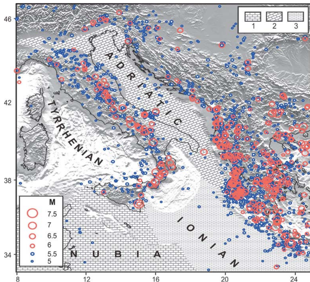
Figure 4. Major earthquakes occurred in the central Mediterranean region since 1600 A.D. 1, 2) Nubia and Adriatic continental domains 3) Ionian oceanic domain. Data from [25]-[32].
