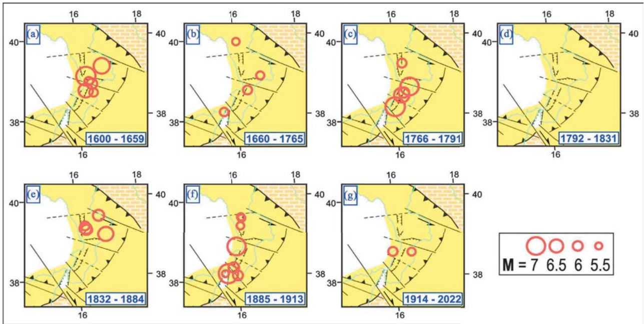
Figure 11. Distribution of major earthquakes ( M \geq 5.5 ) in 7 periods, during which seismicity seems to concentrate in the Northern Calabria ((a), (e)), Central-Southern Calabria ((c), (f)) or to almost disappear ((b), (d), (g)).
