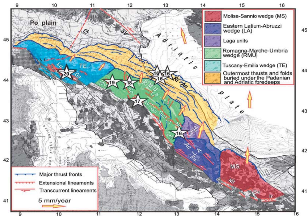
Figure 12. Distribution of main earthquakes (stars and occurrence year) with M \geq 5.5 in the northern Apennines (1916-1920, see Figure 13 for details) after the strong 1915 shock ( M = 7.1 ) in the Fucino fault [32]. Colours identify the outer mobile sectors of the Apennine belt reported on the Geological Map of Italy ([45], modified). Aq = L'Aquila fault, AVT = Alta Valtiberina trough, Be = Benevento fault, Ca = Cagliari fault, Cf = Colfiorito fault, Fa = Fabriano fault, Fu = Fucino fault, Ga = Garfagnana trough, Gi = Giudicarie fault system, Gu = Gubbio fault, Gua = Gualdo Tadino fault, Ir = Irpinia fault, Lu = Lunigiana trough, Mt = Matese fault, Mu = Mugello trough, No = Norcia fault, Ro = Romagna fault, Ri-An = Rimini-Ancona thrust front. The yellow arrows indicate the kinematic field [33] [46].
