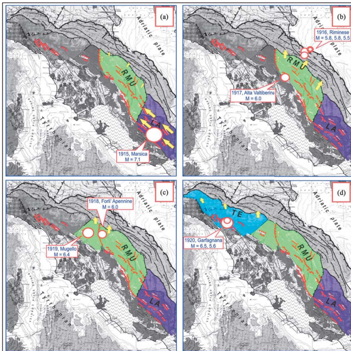
Figure 13. Tentative reconstruction of the short-term kinematic pattern in the northern Apennines (reported on the Geological Map of Italy [45], modified) that was triggered by the earthquakes occurred from 1915 to 1920 [32]. (a) The Fucino event with more than 1 m of sliding at the fault [47] decouples the LA block (violet) from the inner Tyrrhenian belt triggering the acceleration of this block (yellow arrows) and of the southern RMU wedge (green). (b) The increase of compressional stress at the northern boundary of RMU causes the three Riminese shocks (1916). The displacement allowed by this thrusting favours the motion of this wedge, increasing stress in the AVT trough, where the 1917 earthquake took place. (c) Once decoupled at its outer and inner boundaries, the northern RMU wedge moves faster, favouring its decoupling from the Emilian Apennines, allowed by the Romagna Apennine shock (1918). The previous earthquakes increased stress in the northernmost sector of the RMU wedge (green), causing the Mugello earthquake (1919). (d) The acceleration reaches the Tuscany-Emilia Apennines, causing the activation of the Garfagnana fault (1920).
