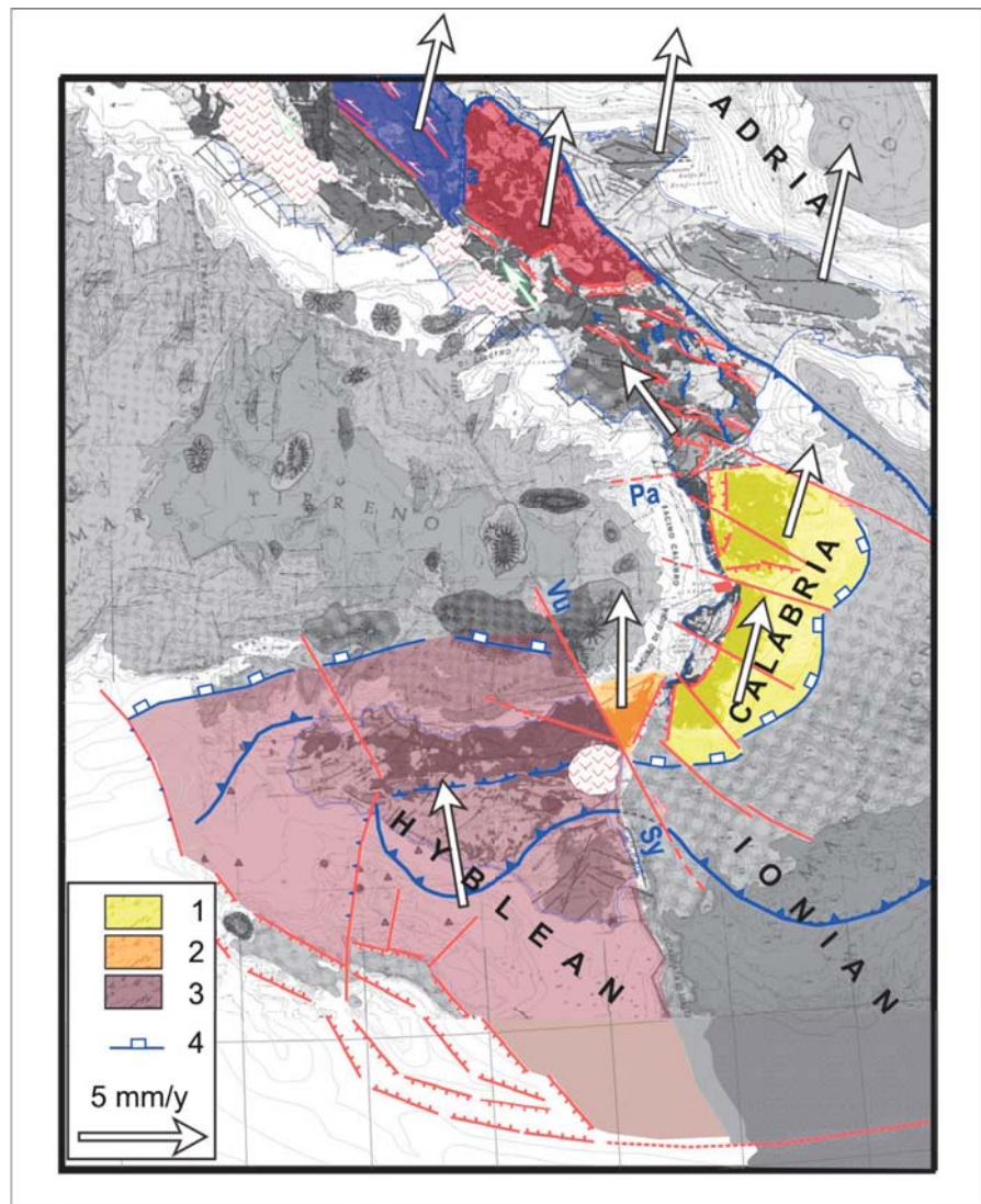
Figure 9. Tectonic-kinematic context in the central Mediterranean region, reported on the Geological Map of Italy ([45], modified). 1) Calabrian wedge 2) Peloritani block 3) Hyblean wedge 4) Outer front of the Alpine units. White arrows indicate the proposed kinematics with respect to Eurasia. The convergence between the confining plates is accommodated by the opposite extrusions of the Calabrian and Hyblean wedges. Pa = Palinuro fault, Vu-Sy = Vulcano-Syracuse fault system. Other symbols as in Figure 5 .
