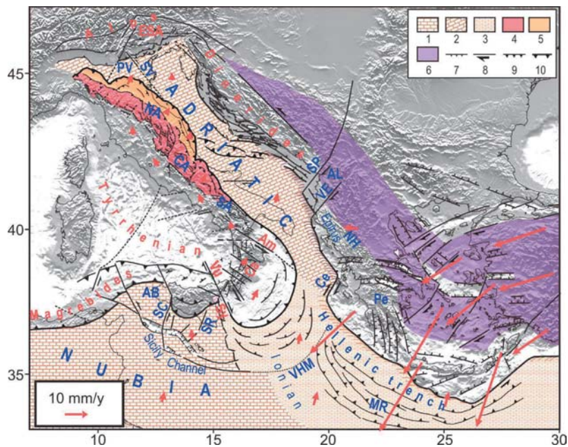
Figure 5. Present tectonic and kinematic settings of the central Mediterranean area. Stressed by the Adriatic plate, the eastern part of the Apennine belt (brown) is undergoing belt-parallel shortening, accommodated by uplift and formation of arcs. 1-2) Nubia and Adriatic continental domains 3) Ionian domain 4) Outer mobile side of the Apennine belt 5) Buried external folds in the Northern Apennines 6) Anatolian-Aegean-Pelagonian belt 7, 8, 9) Tensional, transcurrent and compressional features 10) Outer thrust fronts. Al = Albanides; AB = Adventure block, Am = Amendolara fault, Ca = Calabrian wedge, Ce = Cephalonia fault, ESA = Eastern Southern Alps, MR = Mediterranean ridge, NA, CA, SA = Northern, Central and Southern Apennines, NH = Northern Hellenides, Pe = Peloponnesus; PV = Po Valley; SC = Sciacca fault; SP = Scutari-Pec fault, SR = Scicli-Ragusa fault; SV = Schio-Vicenza fault, VE = Vlora-Elbasan fault; VHM = Victor Hensen-Medina fault system; Vu-Sy = Vulcano-Syracuse fault system. Red arrows indicate the present kinematic field [4] [6] [33] [34].
