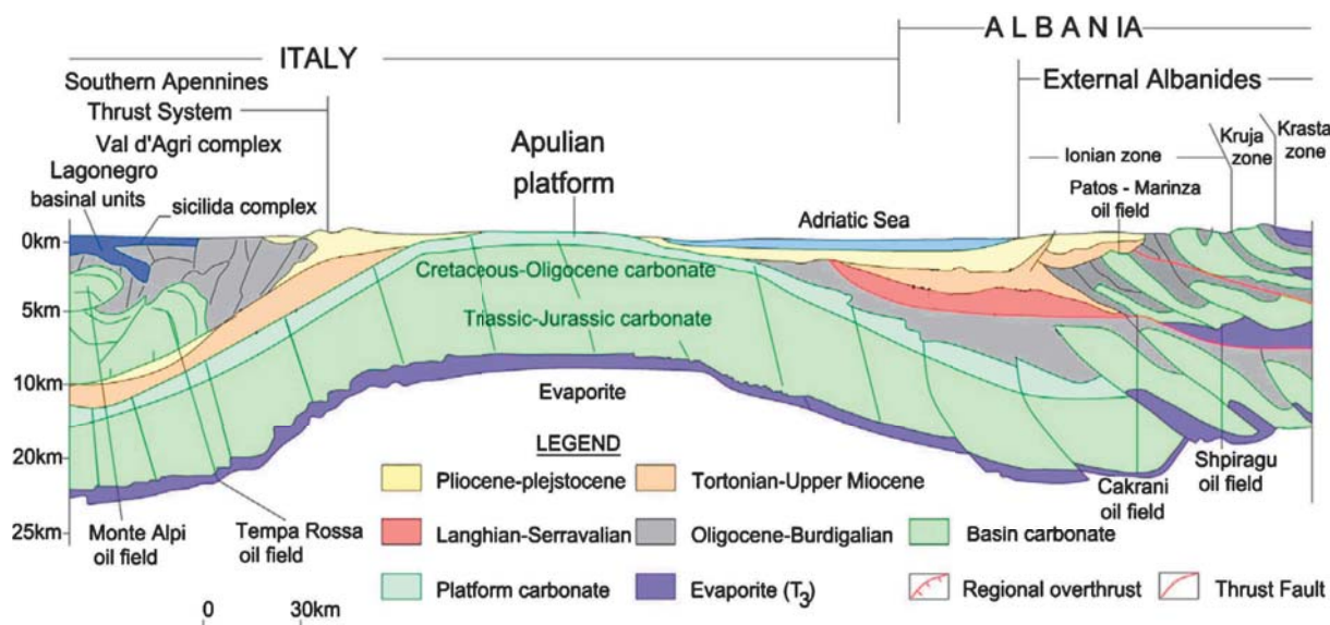
Figure 2. Section across the southern Adriatic domain (From [8], modified). The upward flexure of this domain testifies a strong E-W compression, driven by the convergence between the Anatolian-Aegean-Pelagonian belt and Nubia [4] [5] [6] [9] [10].
