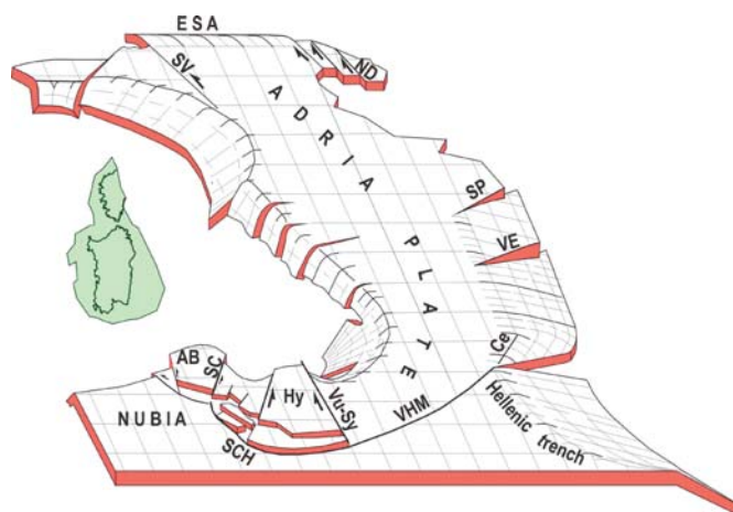
Figure 6. Perspective view of the Adria plate and its buried margins. The shallow structures are shown in Figure 5. AB = Adventure block, Ce = Cephalonia fault, ESA = Eastern Southern Alps, Hy = Hyblean plateau, ND = Northern Dinarides, SC = Sciacca fault, SCH = Sicily Channel fault system, SP = Scutari-Pec fault, SV = Schio-Vicenza fault, VE = Vlora-Elbasan fault, VHM = Victor Hensen-Medina fault system, Vu-Sy = Vulcano-Syracuse fault system.
