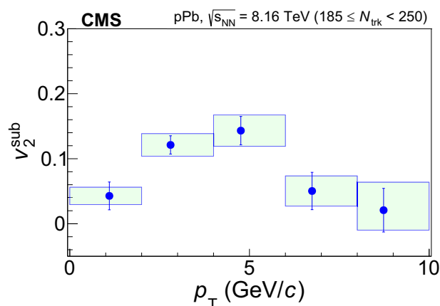
Fig. 2 | Elliptic anisotropy results. The nonflow-effect-subtracted elliptic anisotropy v_2^{\text{sub}} of the f_0(980) is shown as a function of p_T within |y| \lesssim 2.4 in high-multiplicity pPb collisions. The error bars show statistical uncertainties while the shaded areas represent systematic uncertainties.
