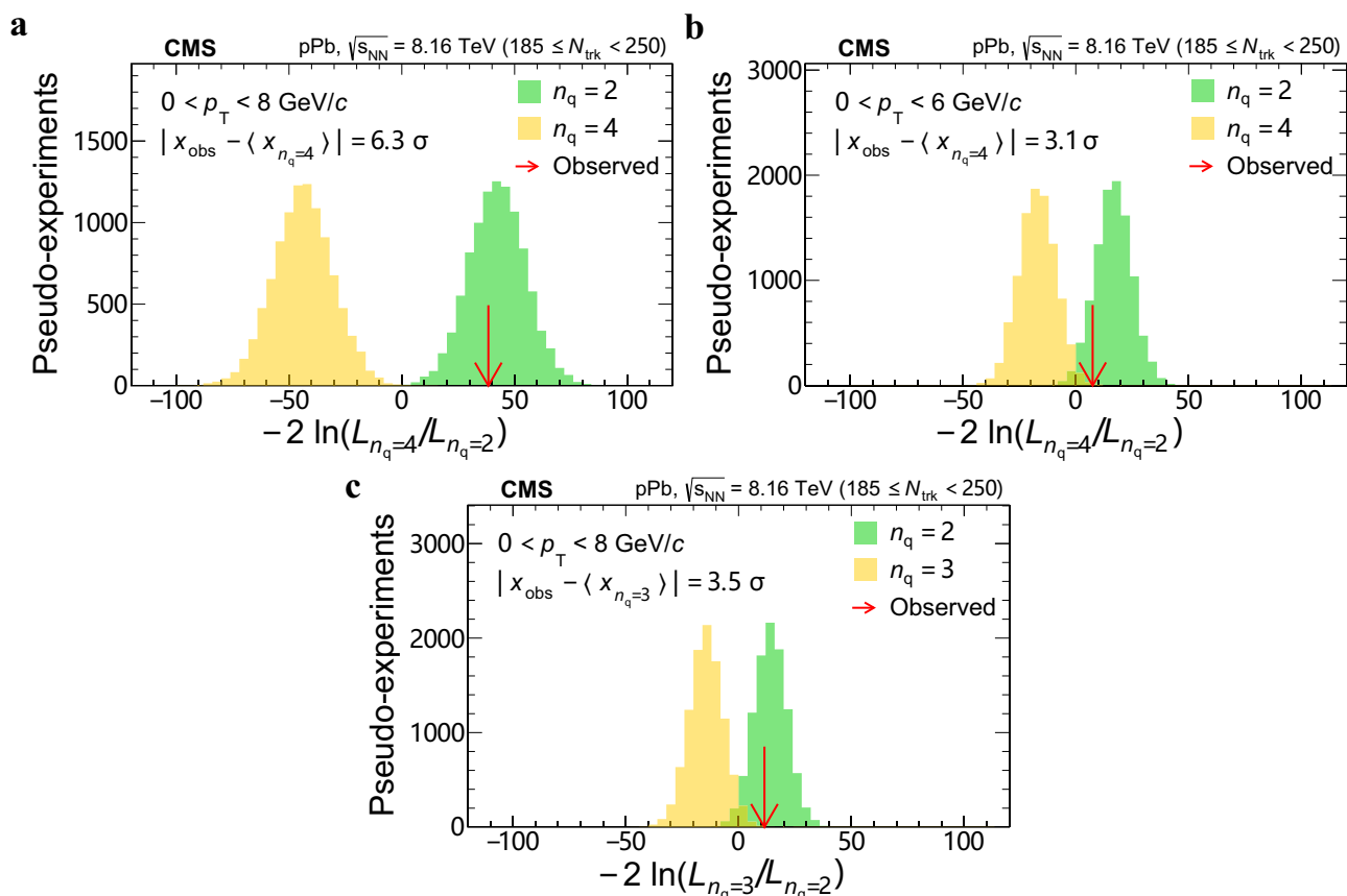
Fig. 9 | Exclusion significances. Same as Fig. 4 but using f_0(980) \nu_2^{\text{sub}} data within the restricted ranges p_T < 8 GeV/c (a) and p_T < 6 GeV/c (b). c The expected log-likelihood ratio distributions for n_q = 2 vs. 3 hypotheses from the pseudo-
