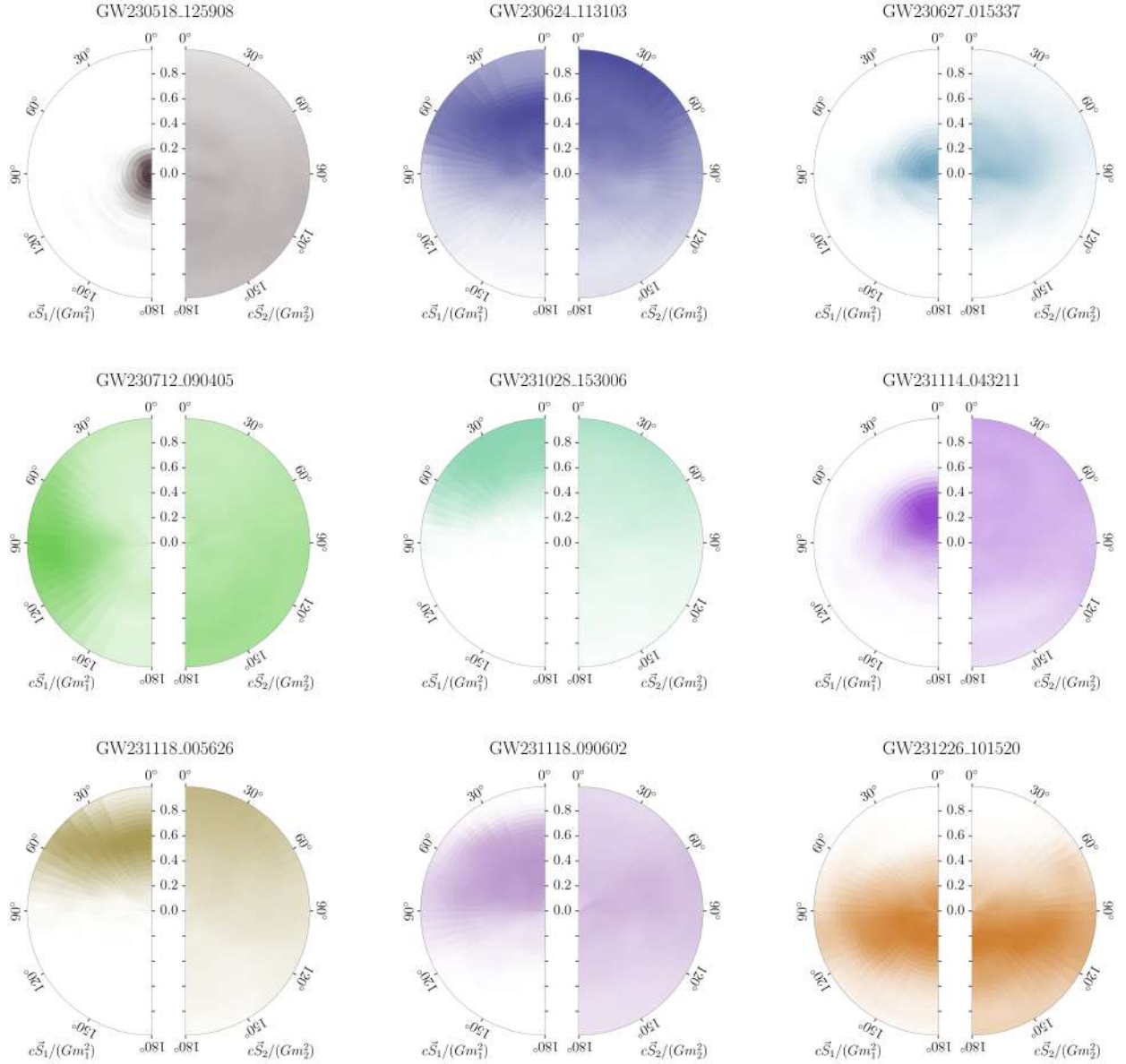
Figure 6. Posterior probability distributions for the dimensionless component spins \chi_1 = cS_1/(Gm_1^2) and \chi_2 = cS_2/(Gm_2^2) (with S_1 and S_2 the spin vectors of the components) relative to the orbital plane, marginalized over azimuthal angles, for candidates GW230518_125908, GW230624_113103, GW230627_015337, GW230712_090405, GW231028_153006, GW231114_043211, GW231118_005626, GW231118_090602, and GW231226_101520. In these plots, the histogram bins are constructed linearly in spin magnitude and the cosine of the tilt angles, such that they contain equal prior probability.
