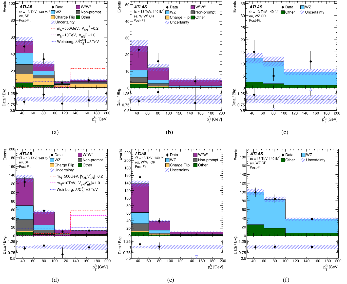
Fig. 2. Distributions of the p_T^{\ell\ell} in (a) the ee SR, (b) the ee same-sign WW CR, (c) the ee WZ CR, (d) the e\mu SR, (e) the e\mu same-sign WW CR, and (f) the e\mu WZ CR. The predicted yields are shown with their best fit normalization and shape from the fit for the SM background-only hypothesis. The shaded area surrounding the background expectation represents the total uncertainties in the predicted yields. The ratios of the observed yields to the total SM predictions are shown by the points in the bottom panels. ‘Other’ includes contributions mainly from the \ell\gamma jj , ZZ and tZq background processes. Benchmark signal predictions are shown as hatched lines. The last bin includes the overflow.
