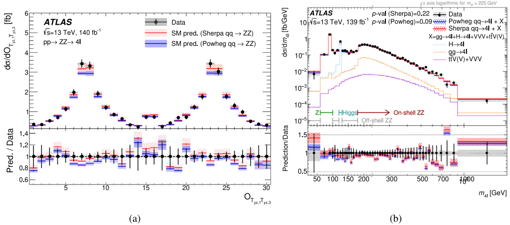
Fig. 28. (a) Differential ZZ \rightarrow 4l cross-section as a function of the Optimal Observable O_{T_{yz,1}T_{yz,3}} [213] and (b) 4l cross-section as a function of m_{4l} [208]. The lower panels show the ratios of the predictions [6,195] to the data.
