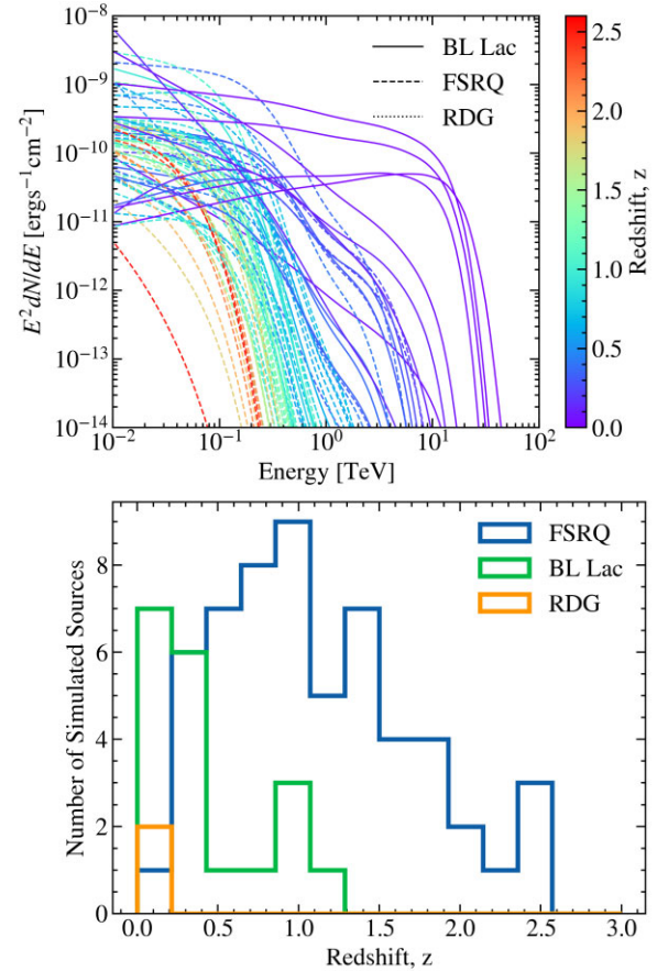
Figure 7. Simulation inputs for the Blazar Detectability Simulation . Top panel: Spectral models of the blazars used as inputs in the simulation. The spectral model is plotted after accounting for absorption due to the EBL according to each source's redshift. Labels correspond to source classes, with 'RDG' indicating Radio Galaxies. Bottom panel: Redshift distribution of the simulated sources by blazar type.
