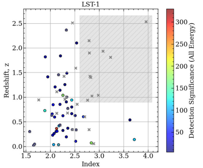
Figure 9. Same as Fig. 8, but for detection significance with all energies. The x-axis shows the photon index before EBL absorption, as used as input to the simulations. The horizontal axis represents the spectral index. The grey shaded area corresponds to the region that will not be detectable by LST-1.
