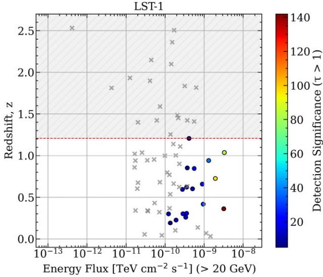
Figure 8. AGN detectability simulation results with a 1.0(1+z) TeV cutoff in all intrinsic spectrum. The color corresponds to detection significance with \tau > 1 . The x-axis represents the integrated energy flux above 20 GeV. Horizontal and vertical axes represent energy flux and source redshift, respectively. The red-dashed line shows the most distant detectable source found in this simulation. The grey shaded area shows the region where AGNs cannot be detected with LST-1.
