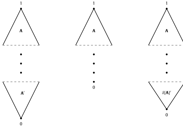
Fig. 1. Respectively: a disconnected 5-rotation, a 5-lifting, and a generalized 5-rotation of a CIRL \mathbf{A} .
