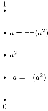
Fig. 2. \text{Rot}_2^\delta(\mathbf{W}_3) from Example 2.6.
