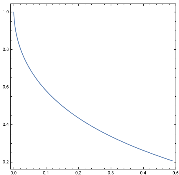
Fig. 1 Plot of 1/\eta_{\alpha,2}(5) for \alpha \in [0, 0.5]
