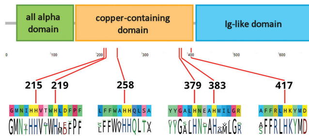
FIGURE 4. Schematic overview of the domain organization of Eusirus cf. giganteus clade g3 hemocyanin. A detail of the six histidine residues expected to be involved in copper binding is provided (His215, His219, His258, His379, His383, His417), along with the consensus sequence of the neighboring residues in crustacean hemocyanin sequences deposited in UniProtKB.
