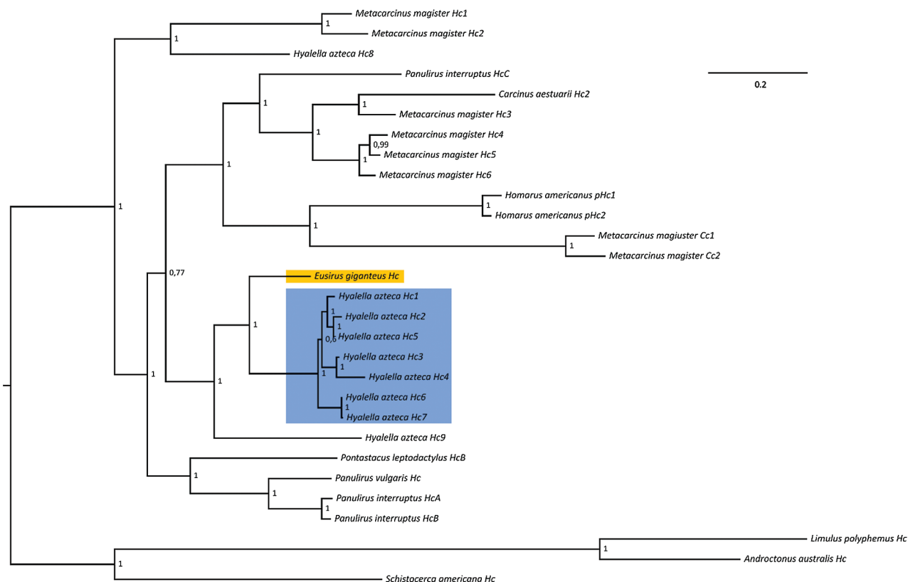
FIGURE 5. Bayesian phylogeny of crustacean hemocyanins. The placement of Eusirus giganteus hemocyanin is highlighted with an orange background. The cluster of paralogous hemocyanin genes from the amphipod Hyalella azteca is highlighted with a blue background. Posterior probability values are shown close to each node. Hc: hemocyanin; Cc: cryptocyanin; pHc: pseudo-hemocyanin.
