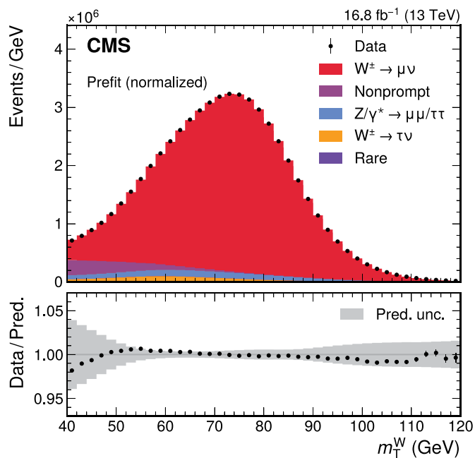
Extended Data Fig. 2 | Measured and predicted m_T distributions in Z \rightarrow \mu\mu and W \rightarrow \mu\nu events, after calibrating u_T . Given that m_T^W is an input variable, the extended ABCD method does not give suitable predictions for the m_T^W distribution. Therefore, the nonprompt background contribution to W boson production is estimated from the QCD multijet simulation. The predictions are those prior to the fit to data. The total uncertainties (statistical and systematic)
