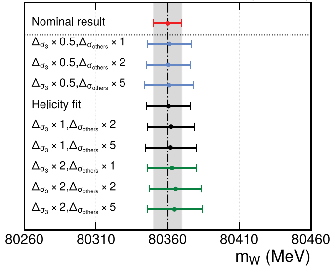
Extended Data Fig. 8 | The W boson mass measured with the helicity fit for different scaling scenarios of the prefactor helicity cross section uncertainties, denoted by \Delta_{\sigma_3} and \Delta_{\sigma_{\text{others}}} for the \sigma_3 and the other components, respectively. The points are grouped and colored according to the scaling of \sigma_3 . The black line indicates the nominal result, with its uncertainties shown by the gray band.
