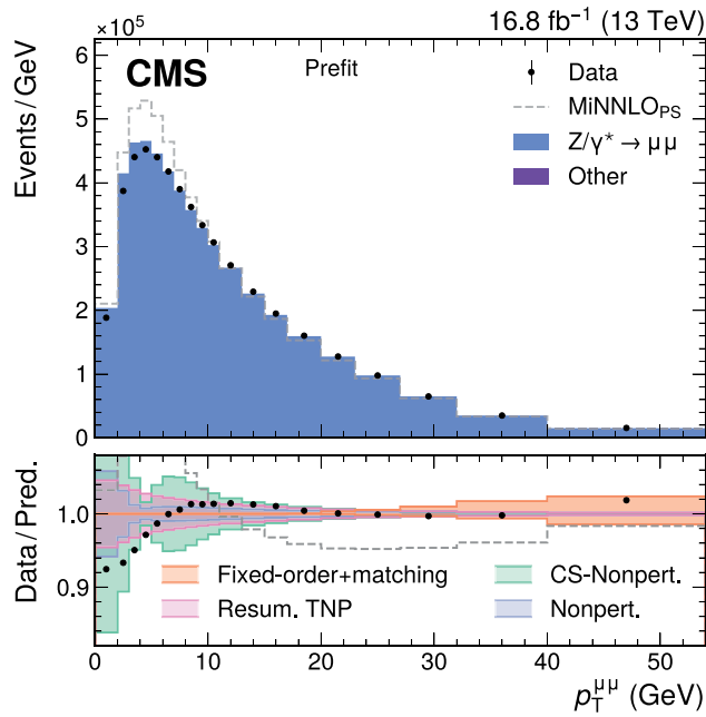
Extended Data Fig. 5 | Measured and simulated p_T^{\mu\mu} (left) and p_T^\mu (right) distributions in selected Z \rightarrow \mu\mu events. The standalone uncorrected MiNNLO _{PS} predictions are shown by the dashed gray line. The nominal predictions (blue) correct the POWHEGMiNNLO _{PS} p_T^\mu with SCETLIB+DYTURBO at N ^3 LL+NNLO, as described in the text. The vertical bars represent the statistical uncertainties in the data. The bottom panel shows the ratio of the number of events observed in data to that of the total nominal prediction, as well as the relative impact of
