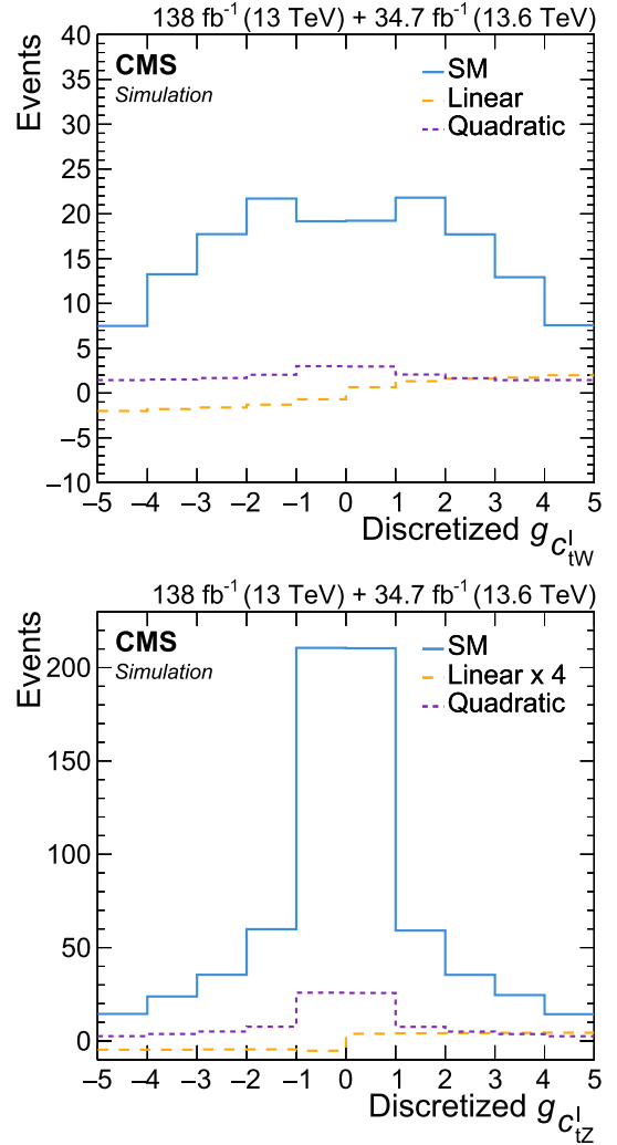
Fig. 2. Upper (lower): Distribution of the discretized g_{c_{iW}^I} ( g_{c_{iZ}^I} ) for events in the c_{iW}^I -like ( c_{iZ}^I -like) category in tZq ( \bar{t}tZ ) events. The contributions from the SM, linear, and quadratic terms when each Wilson coefficient is set to unity are plotted separately. For better visibility the interference contribution in the c_{iZ}^I -like category has been scaled by a factor of 4.
