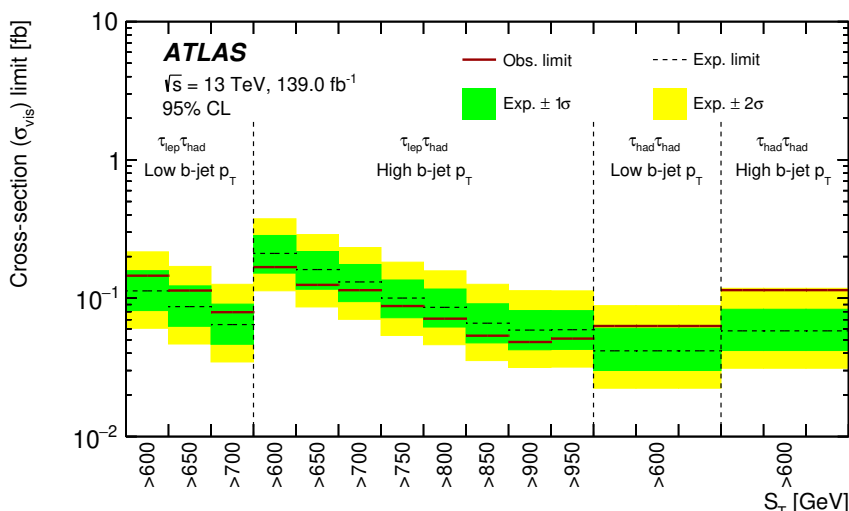
Figure 11. Observed (solid line) and expected (dashed line) 95% upper limits on the visible cross-section, \sigma_{vis} , obtained from the model-independent search by a signal-plus-background fit in the high and low b -jet p_T signal regions for the \tau_{lep}\tau_{had} and \tau_{had}\tau_{had} channels.
