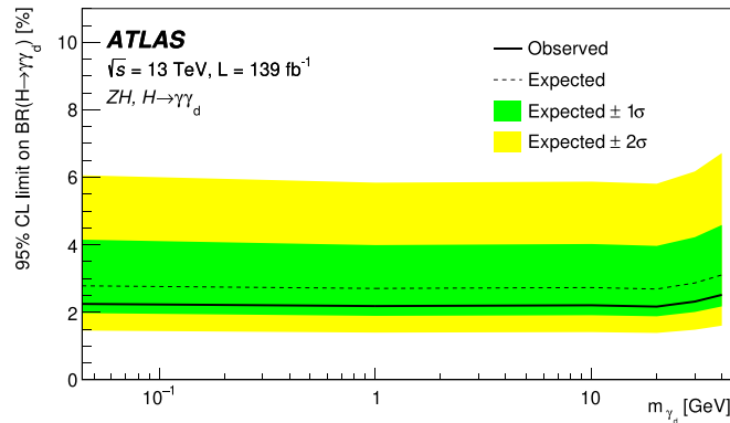
Fig. 50. H \rightarrow \gamma\gamma_d : Observed and expected exclusion limits on B(H \rightarrow \gamma\gamma_d) at 95% CL as function of the \gamma_d mass. Source: The figure is taken from Ref. [134].
