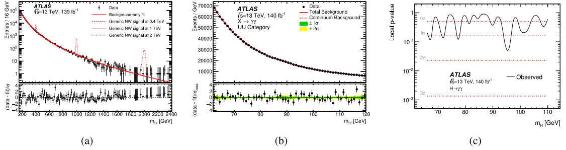
Fig. 21. H \rightarrow \gamma\gamma : (a) The observed diphoton mass and a background-only fit for the high mass search. Various signal hypotheses are overlaid for illustration. (b) The \gamma\gamma mass for the intermediate mass search in the category where both photons are unconverted. (c) The p -value for the model-dependent analysis in the intermediate mass search.
