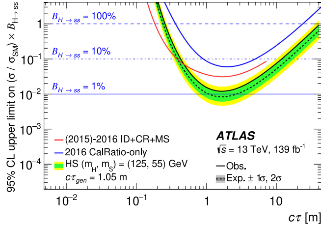
Fig. 57. \Phi \rightarrow SS \rightarrow \text{LLP} : 95% CL expected and observed limits on the branching fraction of SM Higgs bosons to pairs of neutral LLPs ( B_{H \rightarrow ss} ), as well as a comparison with the results from previous ATLAS searches [179,180]. Source: The figure is taken from Ref. [144].
