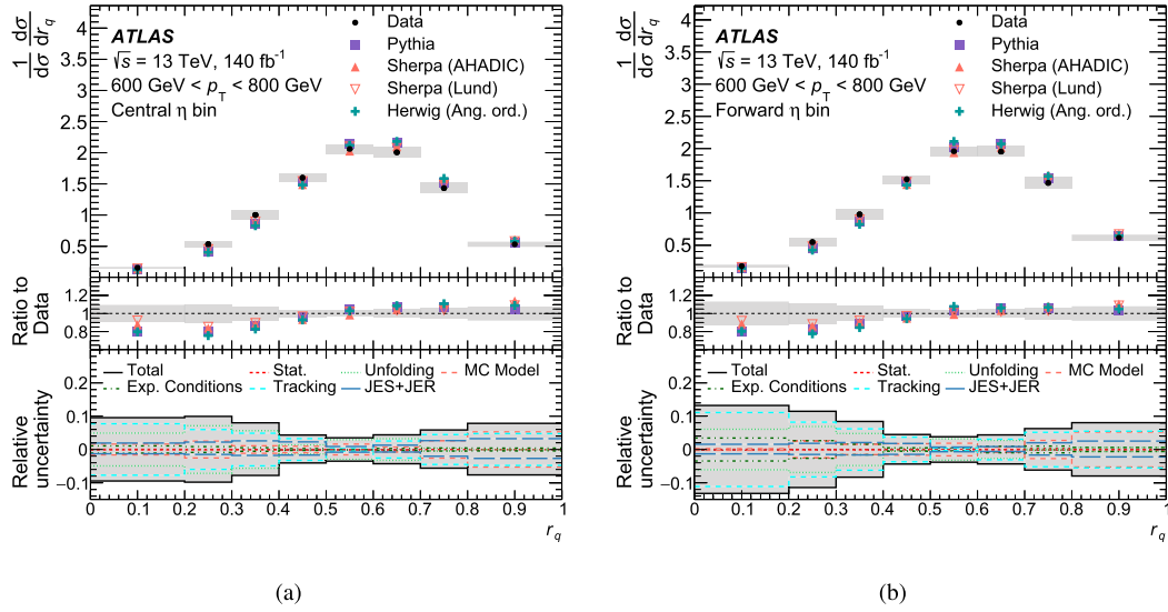
Fig. 1. The unfolded central (a) and forward (b) normalized differential cross-sections as a function of r_q for data compared to predictions from several MC generators. The grey uncertainty band shows the combined statistical and systematic uncertainties on the measurement. The bottom panel shows the breakdown of the uncertainties grouped by their sources. In particular, the ‘Exp. Conditions’ group includes uncertainties related to the overlaid pileup events and potential biases due to differences between disabled modules of the Tile calorimeter.
