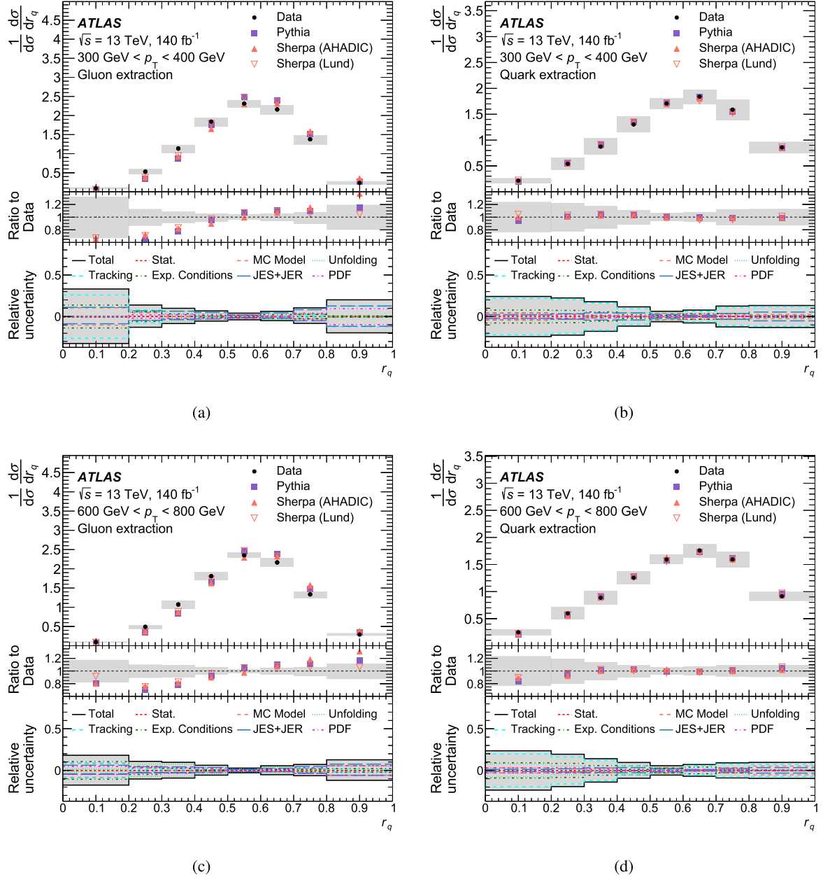
Fig. 5. The demixed (a, c) gluon and (b, d) quark interpretation of the unfolded r_q cross-sections for (a, b) 300 \text{ GeV} < p_T < 400 \text{ GeV} , and (c, d) 600 \text{ GeV} < p_T < 800 \text{ GeV} for data compared to predictions from several MC generators. The grey uncertainty band shows the combined statistical and systematic uncertainties on the measurement. The bottom panel shows the breakdown of the uncertainties grouped by their sources. In particular, the ‘Exp. Conditions’ group includes uncertainties related to the overlaid pileup events and potential biases due to differences between disabled modules of the Tile calorimeter.
