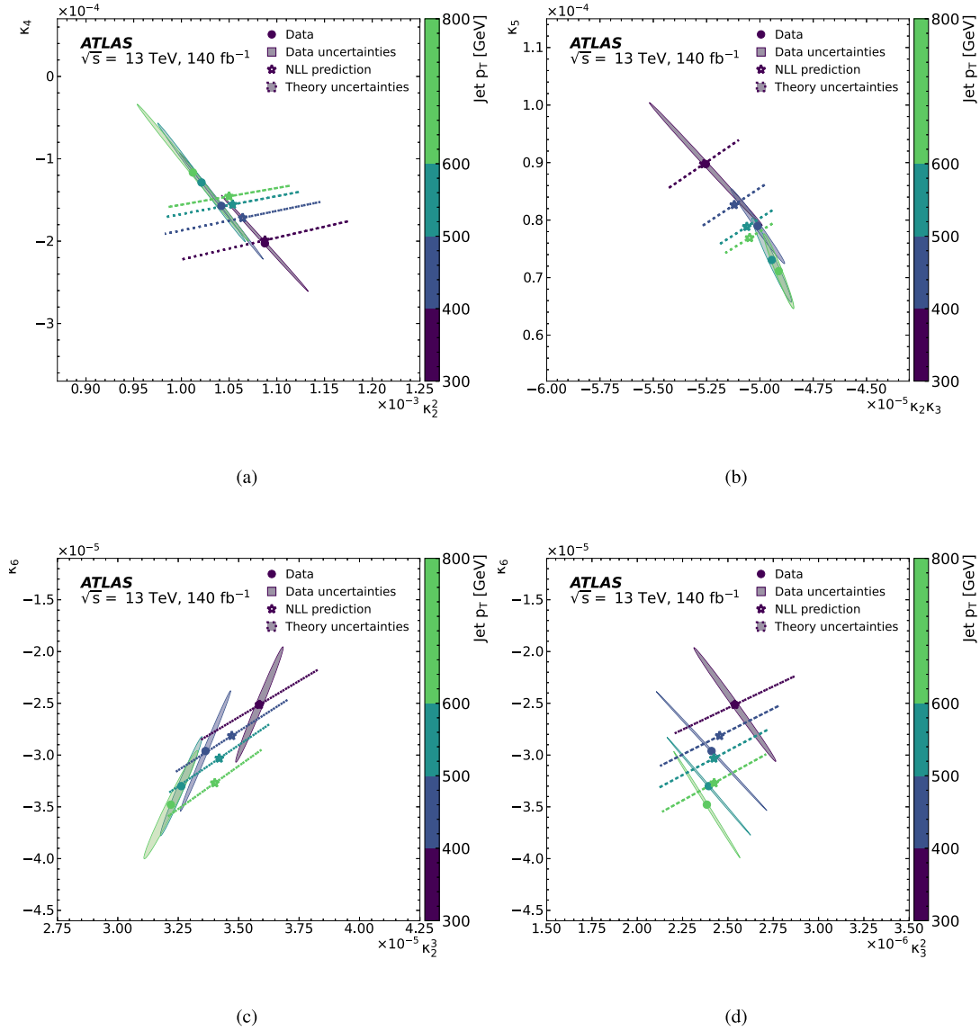
Fig. 3. Non-trivial RG flow relationship between higher-order cumulants and products of lower-order ones coming from the non-linearity of the track function evolution. The relationship between (a) \kappa_4 and \kappa_2^2 , (b) \kappa_5 and \kappa_2\kappa_3 , (c) \kappa_6 and \kappa_2^3 , and (d) \kappa_6 and \kappa_3^2 are shown for different bins of the particle-level jet p_T . The ellipses correspond to the 68% confidence regions based on the combined statistical and systematic uncertainty (data with solid boundaries) and scale variations (theory with dotted boundaries).
