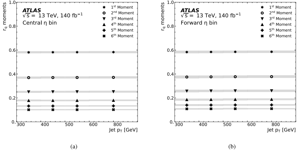
Fig. 2. The first six moments of the unfolded (a) central and (b) forward r_q distributions in jet p_T bins. The grey uncertainty band shows the combined statistical and systematic uncertainties on the measurement.
