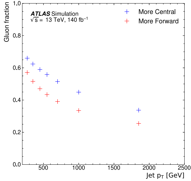
Fig. 4. The gluon fraction obtained from the nominal PYTHIA 8 MC event sample for the more forward and more central of the two dijets as a function of the jet p_T . The cross markers do not include uncertainties in this plot.
