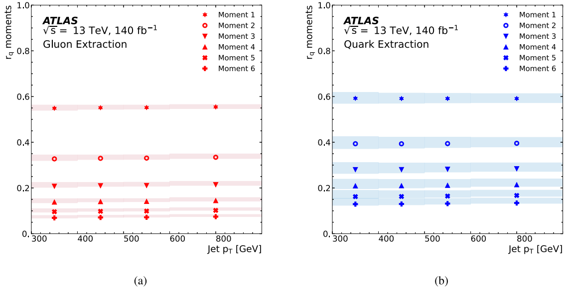
Fig. 6. The first six moments of the demixed (a) gluon and (b) quark r_q distributions in jet p_T bins. The uncertainty bands show the combined statistical and systematic uncertainties on the measurement.
