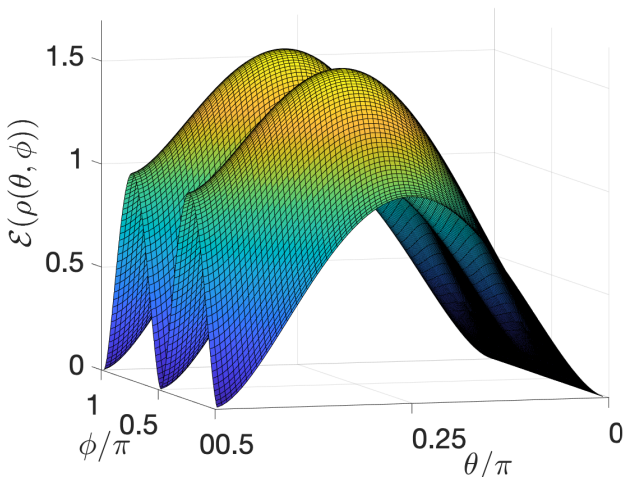
FIG. 7. The figure shows \mathcal{E}(\rho(\theta, \phi)) as a function of \theta/\pi and \phi/\pi given in Eq. (53). The density matrix is associated with the states (51), \rho(\theta, \phi) = |s, \theta, \phi\rangle_{22}\langle s, \theta, \phi| in the case M = 2 .
