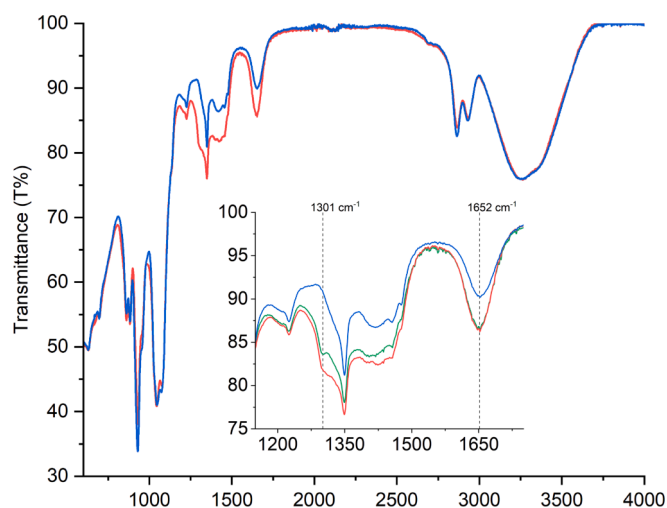
Fig. 11. ATR-FTIR spectra for EG/KOH/BA (3:1:1) before (blue) and after (red) absorption, and after desorption (green). The inset shows the magnification of the spectra in the 1150–1700 \text{cm}^{-1} region. The peaks at 1301 and 1652 \text{cm}^{-1} are marked with dotted lines.
