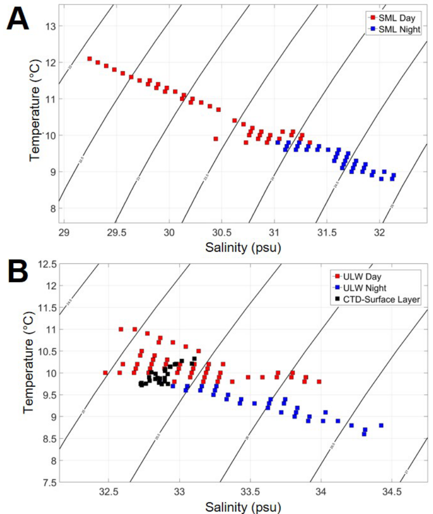
Fig. 5. Temperature–salinity ( T – S ) diagram of (a) the SML and (b) the ULW and at the surface layer CTD (1.3–2 m depth) during cycle 03. Day and night measurements for SML and ULW are shown in red and blue, respectively.
