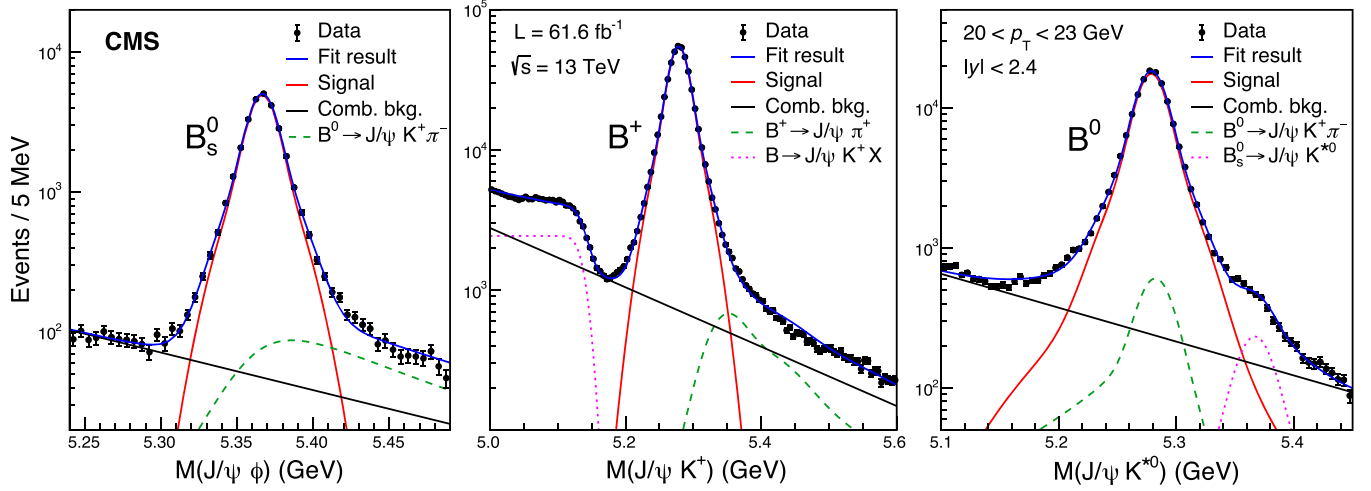
FIG. 1. The J/\psi\phi , J/\psi K^+ , and J/\psi K^{*0} invariant mass distributions for B meson candidates with 20 < p_T < 23 GeV, and associated fits as described in the text.
