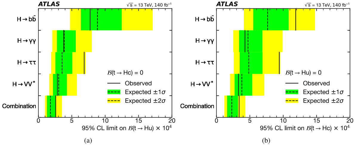
Fig. 15. 95% CL upper limits on (a) B(t \rightarrow Hu) and (b) B(t \rightarrow Hc) for the individual ATLAS searches based on the full Run 2 dataset, as well as their combination (assuming (a) B(t \rightarrow Hc) = 0 and (b) B(t \rightarrow Hu) = 0 ). The observed limits (solid lines) are compared with the expected (median) limits under the background-only hypothesis (dotted lines). The surrounding shaded bands correspond to the 68% and 95% CL intervals around the expected limits, denoted by \pm 1\sigma and \pm 2\sigma , respectively. Figures taken from Ref. [264].
