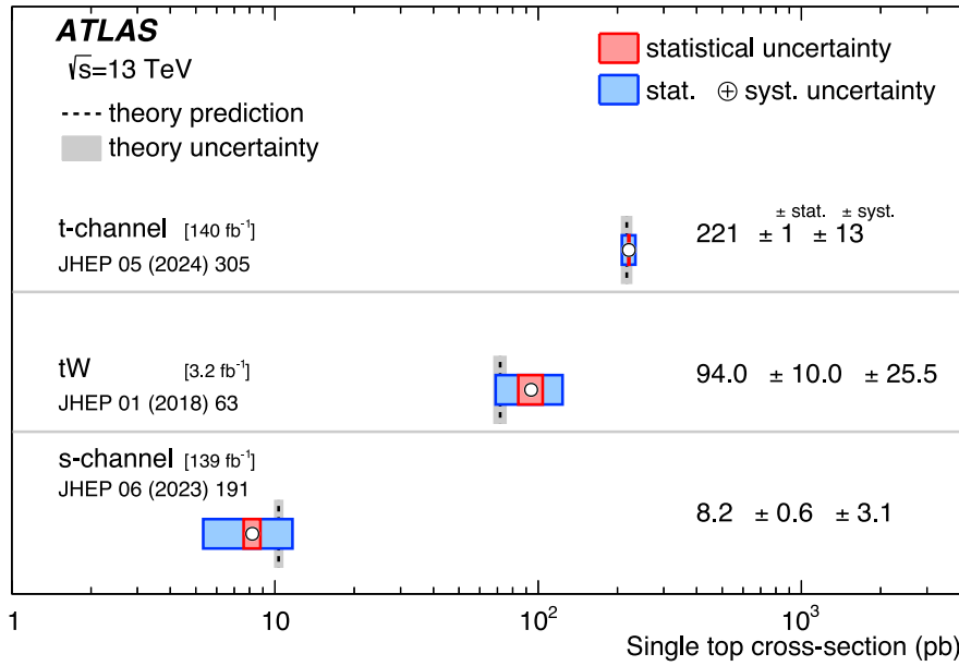
Fig. 8. Summary of the \sqrt{s} = 13 TeV single-top-quark cross-section measurements, compared with the corresponding theoretical expectations. The values are quoted for m_t = 172.5 GeV. The theory predictions are taken from Refs. [107] ( t -channel), [131] ( tW ) and [124] ( s -channel).
