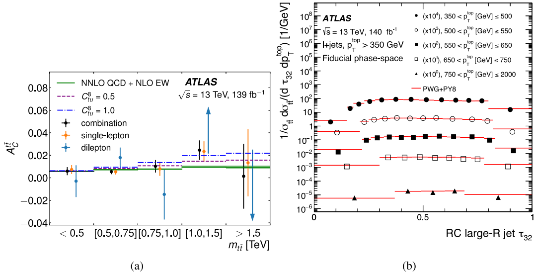
Fig. 14. (a) Unfolded differential charge asymmetry A_C^t as a function of the invariant mass of the reconstructed top-quark pair [225]. (b) Particle-level differential t\bar{t} production cross-section as a function of \tau_{32} for several intervals of top-quark transverse momentum, comparing data measurements with predictions [246].
