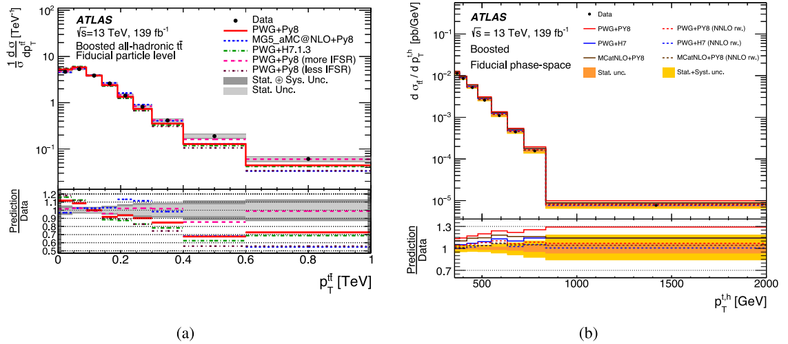
Fig. 5. Two examples of ATLAS differential t\bar{t} cross-section measurements. (a) Normalised particle-level t\bar{t} -system transverse momentum distribution extracted in all-hadronic boosted final states, compared with a number of NLO+PS MC predictions [98]. (b) Particle-level transverse momentum distribution of hadronically decaying top quarks measured in the lepton-plus-jet boosted channel, compared with MC predictions, including predictions where a reweighting of top-quark kinematics is performed to match higher-order fixed-order calculations (see text for more details) [97].
