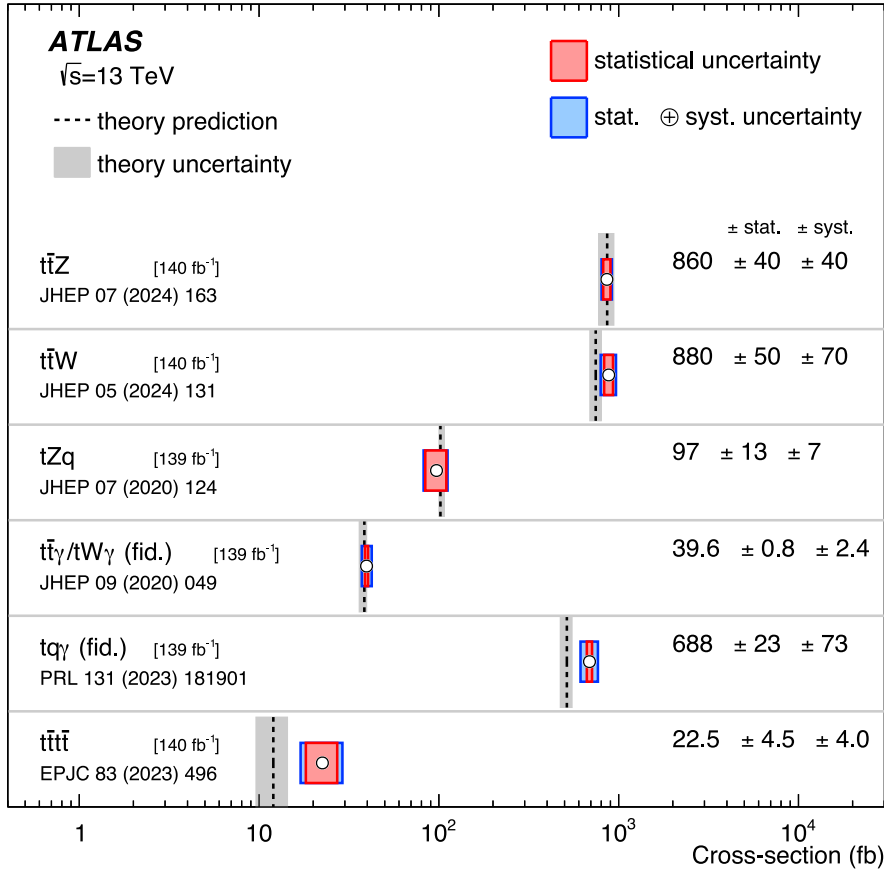
Fig. 10. Summary of the \sqrt{s} = 13 TeV top+X cross-section measurements and comparison with the corresponding theoretical expectations. The fiducial region used to measure the t\bar{t}\gamma cross-section requires one electron, one muon, two b -jets and one photon at parton level. The tq\gamma fiducial region is defined by requiring one electron or muon, at least one photon and at least one b -tagged jet at particle level.
