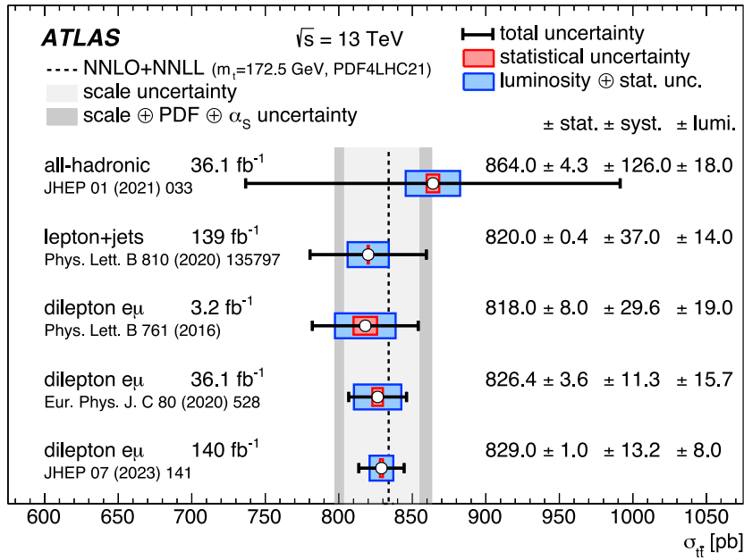
Fig. 3. Summary of ATLAS inclusive t\bar{t} cross-section measurements at \sqrt{s} = 13 TeV based on Run 2 data, compared with the exact NNLO QCD calculation complemented with NNLL resummation (Top++2.0), obtained using the PDF4LHC21 PDF set and with the QCD renormalisation and factorisation scales set to \mu_R = \mu_F = m_t = 172.5 GeV and the strong coupling constant \alpha_s(M_Z) = 0.118 . The theory band represents uncertainties due to renormalisation and factorisation scales, parton distribution functions and the strong coupling constant. The uncertainties in the experimental measurements are broken down into their statistical and systematic components, quoting the uncertainty related to the integrated luminosity separately. The measurements and the theory calculation are quoted for m_t = 172.5 GeV.
