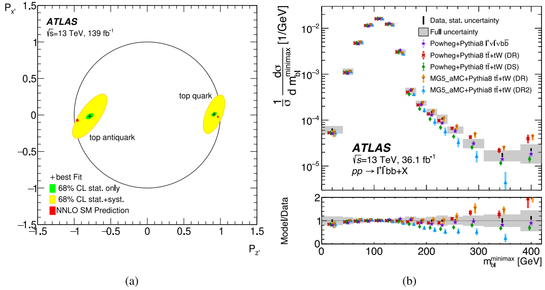
Fig. 7. (a) Observed best-fit polarisation measurements with their statistical (green) and statistical+systematic (yellow) uncertainty contours at 68% CL, plotted on the two-dimensional polarisation parameter space ( P_{z'} , P_{x'} ) [110]. (b) Unfolded normalised differential m_{bt}^{\text{minimax}} cross-section compared with various theoretical models [112].
