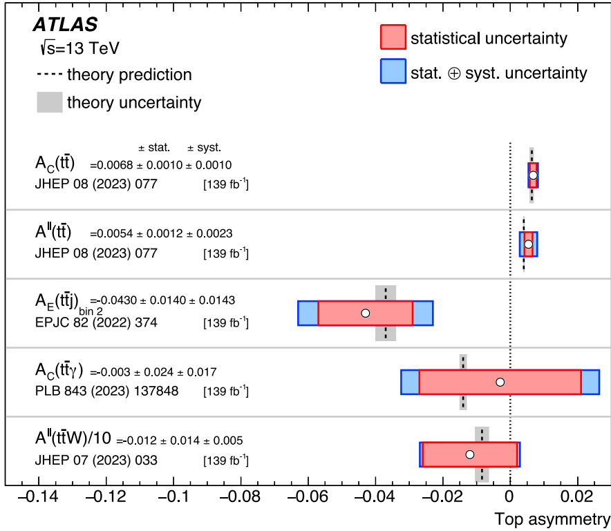
Fig. 13. Summary of the \sqrt{s} = 13 TeV top asymmetry measurements using the full Run 2 dataset: \bar{t}t asymmetry, lepton-based asymmetry, energy asymmetry in the bin with the largest expected asymmetry, and asymmetry in \bar{t}t\gamma and \bar{t}tW events. Each of the results is compared with their corresponding theoretical expectation. The value of the \bar{t}t asymmetry in \bar{t}tW events is shown divided by 10 for display purposes.
