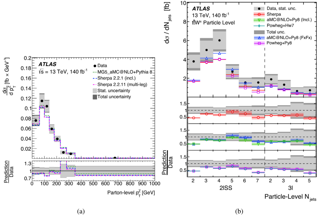
Fig. 9. (a) Absolute differential \bar{t}tZ cross-section measurement as a function of the transverse momentum of the Z boson [147]. (b) Unfolded distribution of the absolute \bar{t}tW cross-section as a function of jet multiplicity [146].
