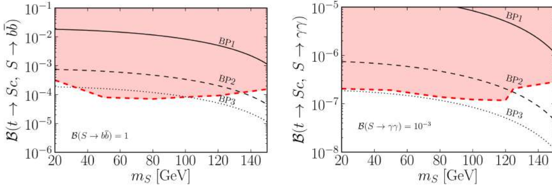
Fig. 76: Branching ratios that can be tested in the b\bar{b} (left) and \gamma\gamma (right) channels at 14 TeV HL-LHC with 3000 \text{ fb}^{-1} (95% CL upper limit is denoted by red dashed line). The three benchmark points, Eq. (142), are denoted with black lines.
