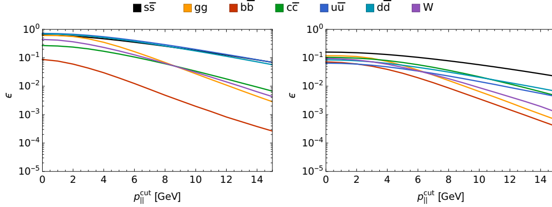
Fig. 69: Efficiencies as function of the cut on p_{||} and for d_0 < 14 \mu\text{m} to reconstruct the different Higgs decay channels and W decays as s\bar{s} event by the described tagger. The left plot shows the CC channel, the right the CN channel.
