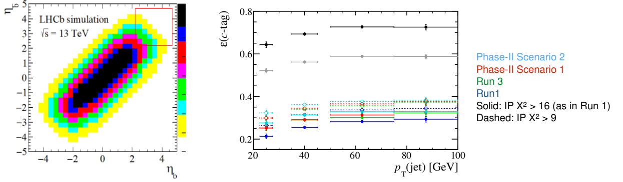
Fig. 68: Left: 2D histogram showing the coverage of the LHCb acceptance for the b\bar{b} pair produced by the Higgs decay in associated production with a W or a Z boson. Right: LHCb c -jet SV-tagging efficiency for different scenarios in the HL-LHC conditions.
