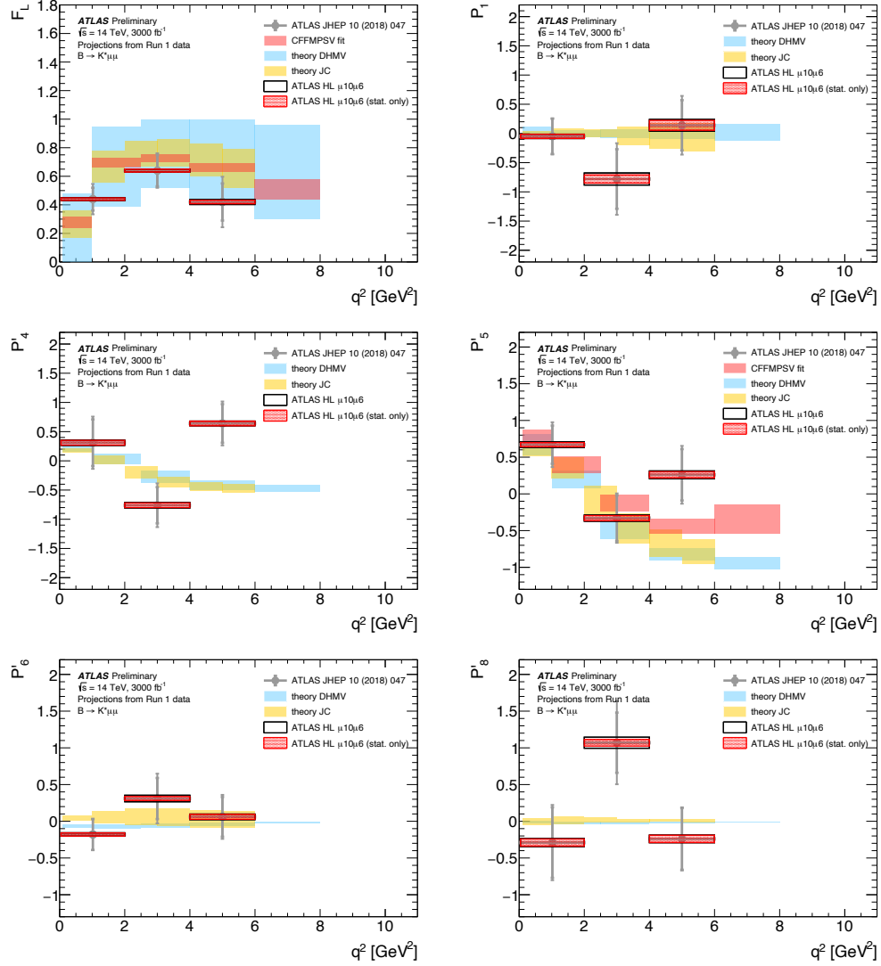
Fig. 52: Projected ATLAS HL-LHC measurement precision in the F_L , P_1 , P_4' , P_5' , P_6' and P_8' parameters for the intermediate \mu 10\mu 6 trigger scenario compared to the ATLAS Run 1 measurement. Alongside theory predictions (CFFMPSV [1120], DHMV [1121], JC [843]) are also shown. Both the projected statistical and the total (statistical and systematic) uncertainties are shown. While the HL-LHC toy-MC were generated with the DHMV central values of the F_L and P_i^{(\prime)} parameters, in these plots the central values are moved to the ATLAS Run 1 measurement for better visualization of the improvement in the precision.
