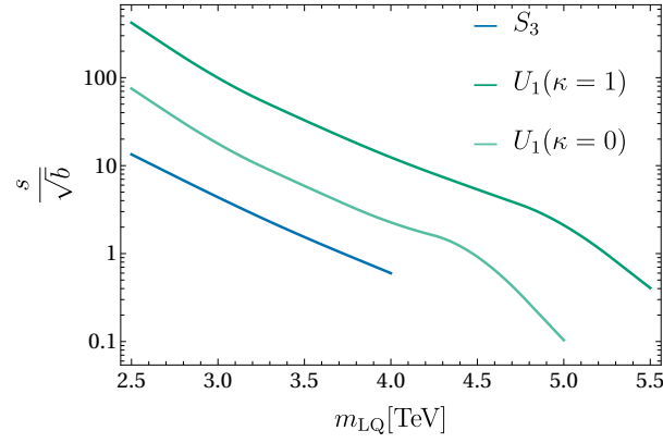
Fig. 99: Expected sensitivity for pair production of scalar ( S_3 ) and vector ( U_1 ) leptoquark at 27 TeV pp collider with an integrated luminosity of 15 ab ^{-1} .
