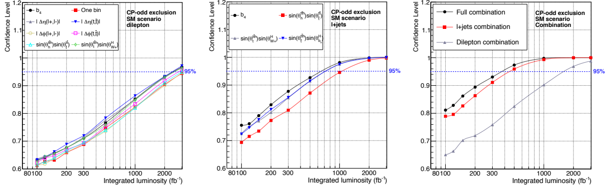
Fig. 74: Expected CL, assuming the SM, for exclusion of the pure CP -odd scenario, \kappa_t = 0, \tilde{\kappa}_t = 1 , as a function of the integrated luminosity. Left: using the t\bar{t}h ( h \rightarrow b\bar{b} ) dileptonic analysis only, middle: using the t\bar{t}h ( h \rightarrow b\bar{b} ) semileptonic analysis only, right: combining observables in each individual channel and combining both channels, treating the observables as uncorrelated. A likelihood ratio computed from the binned distribution of the corresponding discriminant observable was used as test statistic.
