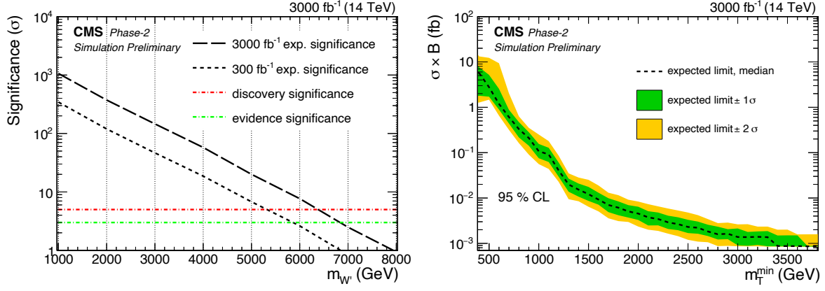
Fig. 98: Left: Discovery significance for SSM W' to tau leptons. Right: Model-independent cross section limit. For this, a single-bin limit is calculated for increasing M_T^{\min} while keeping the signal yield constant in order to avoid including any signal shape information on this limit calculation.
