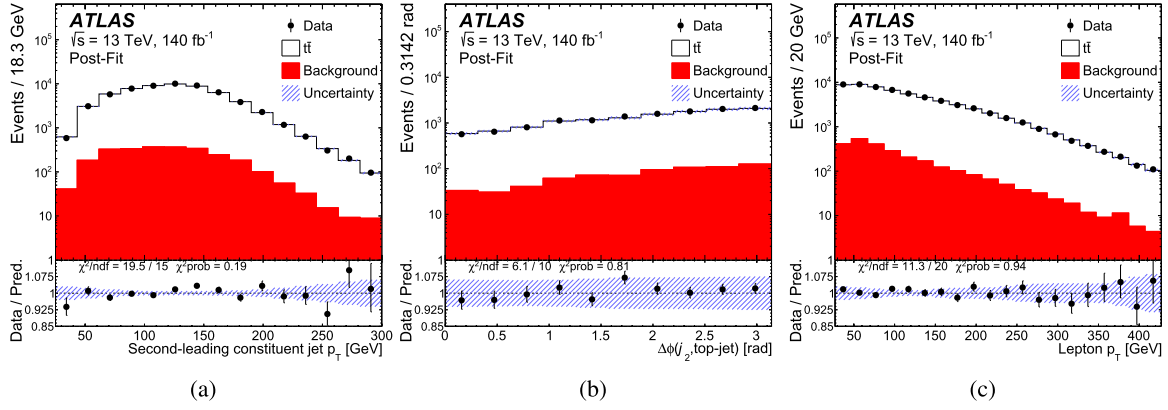
Fig. 4. The distributions of (a) the p_T of the second-leading constituent inside the top-jet, (b) the \Delta\phi between the second-leading additional jet and top-jet (for events including at least two additional jets), and (c) the selected lepton p_T are compared with the prediction of the post-fit model. These distributions do not include the overflow of events that can satisfy the event selection of Section 3. The uncertainty band includes the effect of the systematic uncertainties, including the post-fit correlations and constraints. The bottom panel reflects the agreement between the data and total prediction, where the error bars show the statistical uncertainty of the data. Values of \chi^2 and the number of degrees of freedom (ndf) are provided for each distribution.
