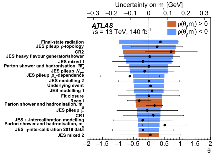
Fig. 3. The contribution of individual NPs, \theta , to the total uncertainty in m_t is shown by the coloured bars and can be read off using the upper x-axis. The red (blue) coloured bars represent NPs that have a positive (negative) correlation with m_t and only NPs that have a contribution to the uncertainty in m_t of more than 0.05 GeV are shown. The fitted values and post-fit uncertainties for these NPs are shown by the points, which refer to the lower x-axis. All modelling uncertainties displayed in the figure correspond to uncertainties in the t\bar{t} process.
