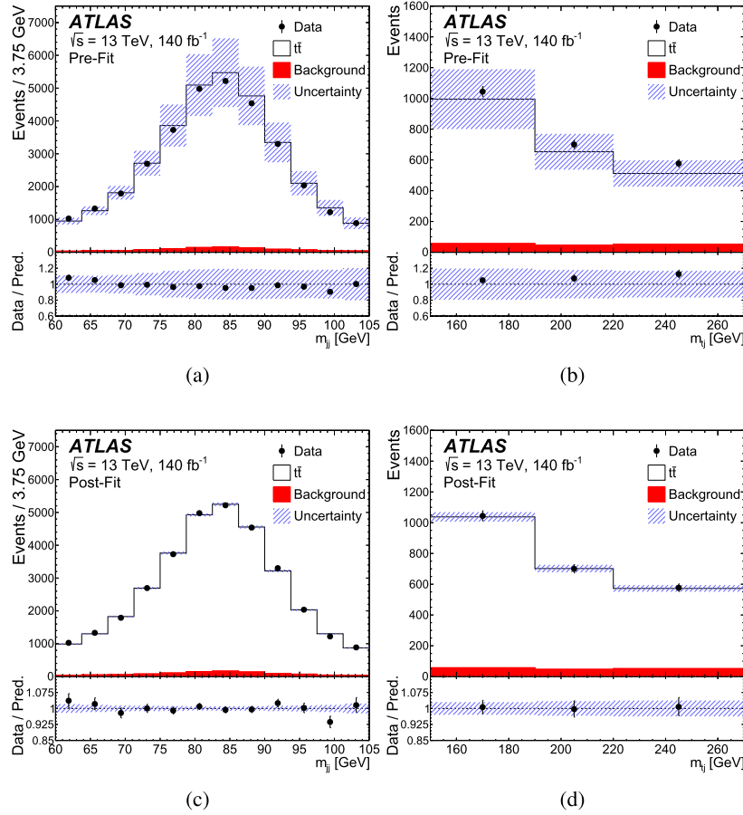
Fig. 2. The pre and post-fit expectations for the m_{jj} and m_{tj} distributions are compared with the data. For the pre-fit case, the t\bar{t} sample corresponds to m_t = 172.5 GeV and is scaled to \mu = 0.856 , which is the ratio of data to theory found in the previous ATLAS cross-section measurement [22]. There is no uncertainty in the pre-fit value of \mu . The uncertainty band represents the total uncertainty in the model and is significantly reduced after the fit. The bottom panel reflects the agreement between the data and total prediction, where the error bars show the statistical uncertainty of the data. This includes the systematic and MC statistical uncertainties and for the post-fit case it also includes the uncertainty on \mu .
