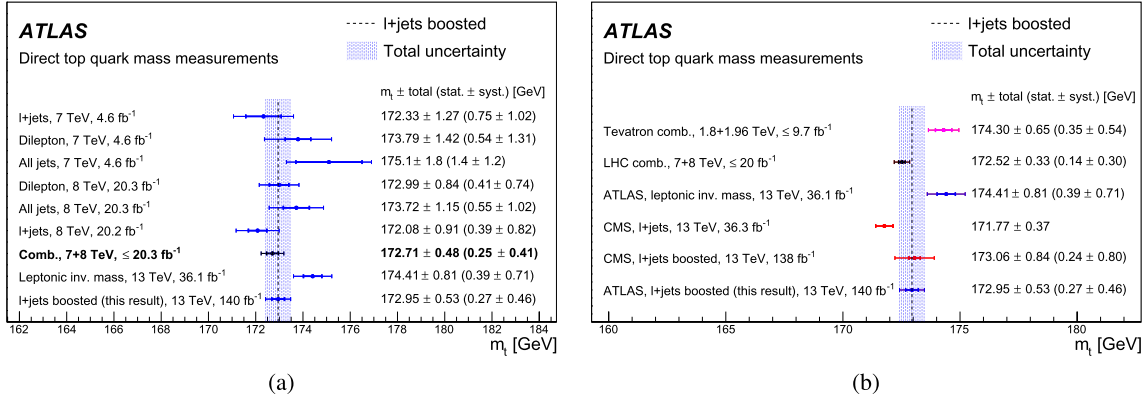
Fig. 6. The measurement of the top quark mass in this Letter is compared with (a) other ATLAS measurements and (b) other precise direct determinations of m_t . The ATLAS combination displayed in bold in (a) is a combination of all the results listed above it. The dashed line and shaded band represent the central value and uncertainty of this measurement, which is also shown as the final measurement point in each plot.
