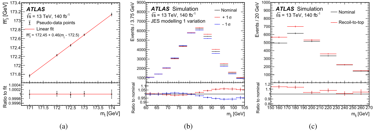
Fig. 1. The dependence of \overline{m}_T on m_t is shown in (a) where the filled pseudo-data points are built from t\bar{t} samples with different values of the top quark mass and the nominal background prediction. For each point, \overline{m}_T is calculated using events in the range of 145 < m_J < 205 GeV. The linear fit to the points is shown by the solid line and the fit parameters are also displayed in (a). (b) Comparison between the m_{jj} distribution expected for the nominal t\bar{t} simulation and the simulation where one of the JES uncertainties is varied to \pm 1\sigma and (c) m_{tj} distribution for the alternative recoil-to-top model used in the top quark decay compared with the nominal t\bar{t} prediction. The error bars show the statistical uncertainty in the MC samples.
