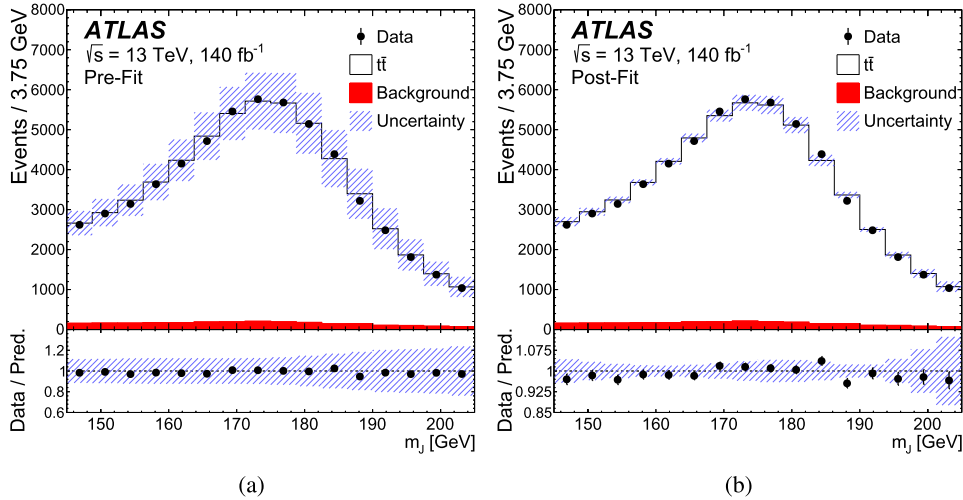
Fig. 5. The (a) pre-fit and (b) post-fit expectations for the m_J distribution are compared with the data. The fit does not contain the distribution of m_J , but only the value of \overline{m_J} . The distribution is shown to illustrate the agreement between data and prediction. For the pre-fit case, the t\bar{t} sample corresponds to m_t = 172.5 GeV and is scaled to \mu = 0.856 , which is the ratio of data to theory found in the previous ATLAS cross-section measurement [22]. There is no uncertainty in the pre-fit value of \mu or m_t . The uncertainty band represents the total uncertainty in the model and is significantly reduced after the fit. The bottom panel reflects the agreement between the data and total prediction, where the error bars show the statistical uncertainty of the data. This includes the systematic and MC statistical uncertainties and for the post-fit case it also includes the uncertainty in \mu and m_t .
